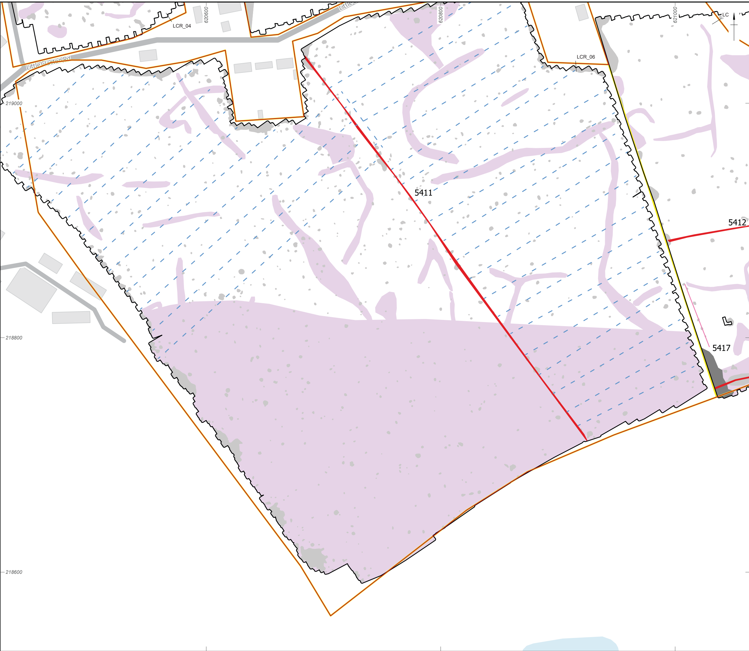
Figure 109: Gradiometer survey results: interpretation (LCR_07, LCR_06, LCR_04)
