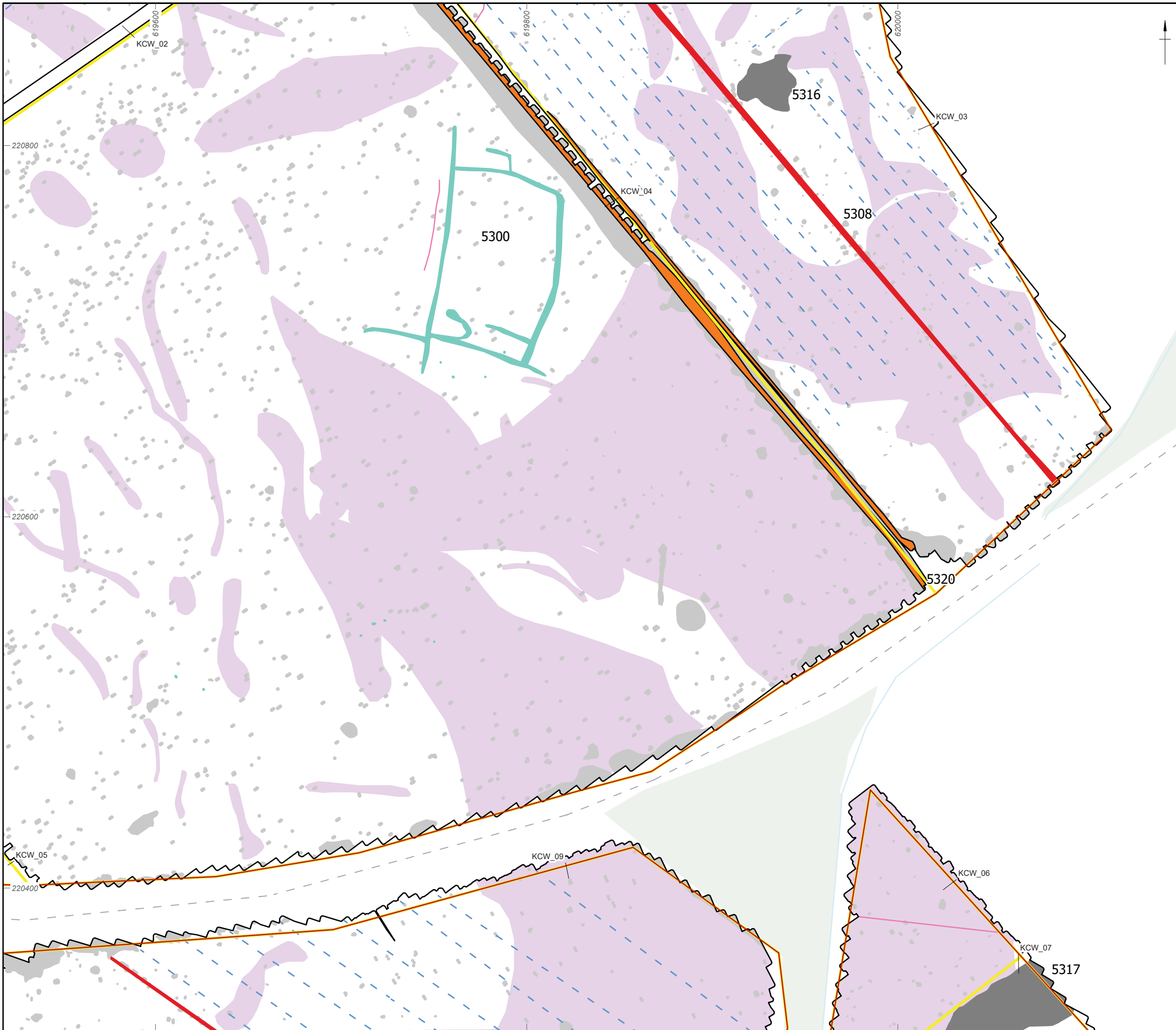
Figure 99: Gradiometer survey results: interpretation (KCW_04, KCW_09, KCW_03, KCW_02, KCW_06, KCW_07, KCW_05)
