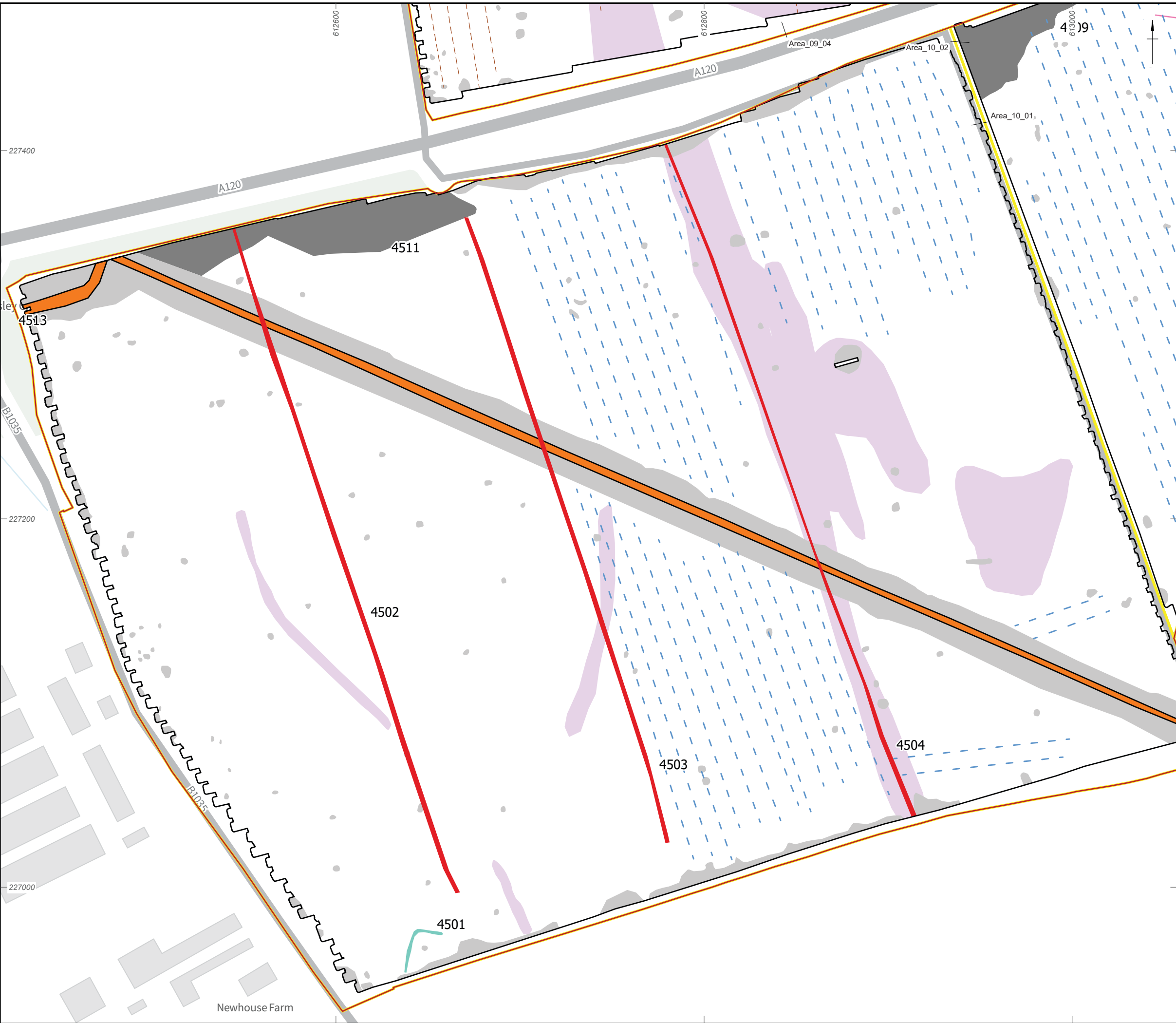
Figure 53: Gradiometer survey results: interpretation (Area_09_04, Area_10_02, Area_10_01)
