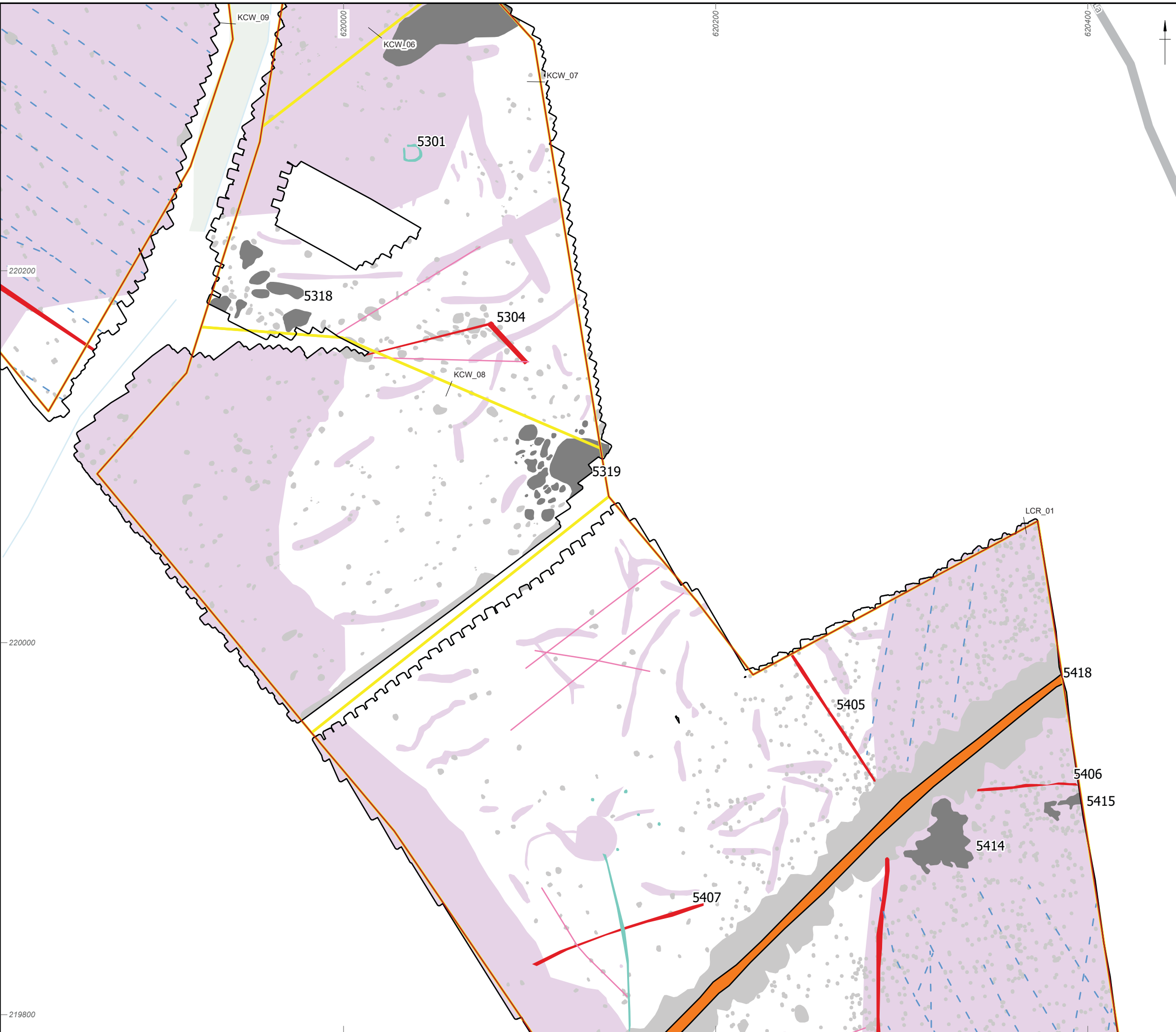
Figure 103: Gradiometer survey results: interpretation (LCR_01, KCW_09, KCW_06, KCW_07, KCW_08)
