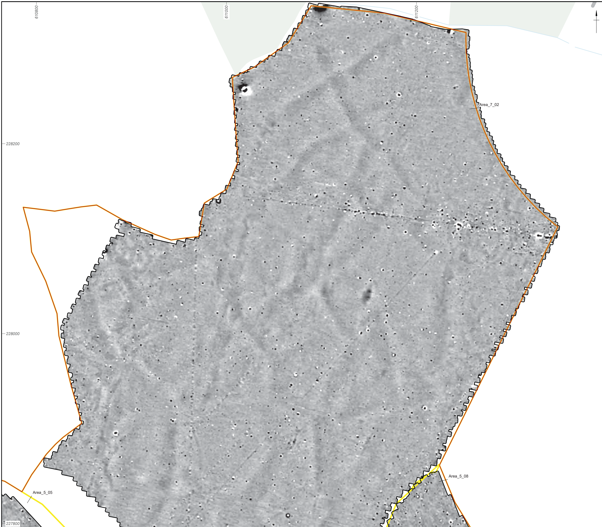
Figure 42: Gradiometer survey results: greyscale plot (Area_5_08, Area_5_05, Area_7_02)
