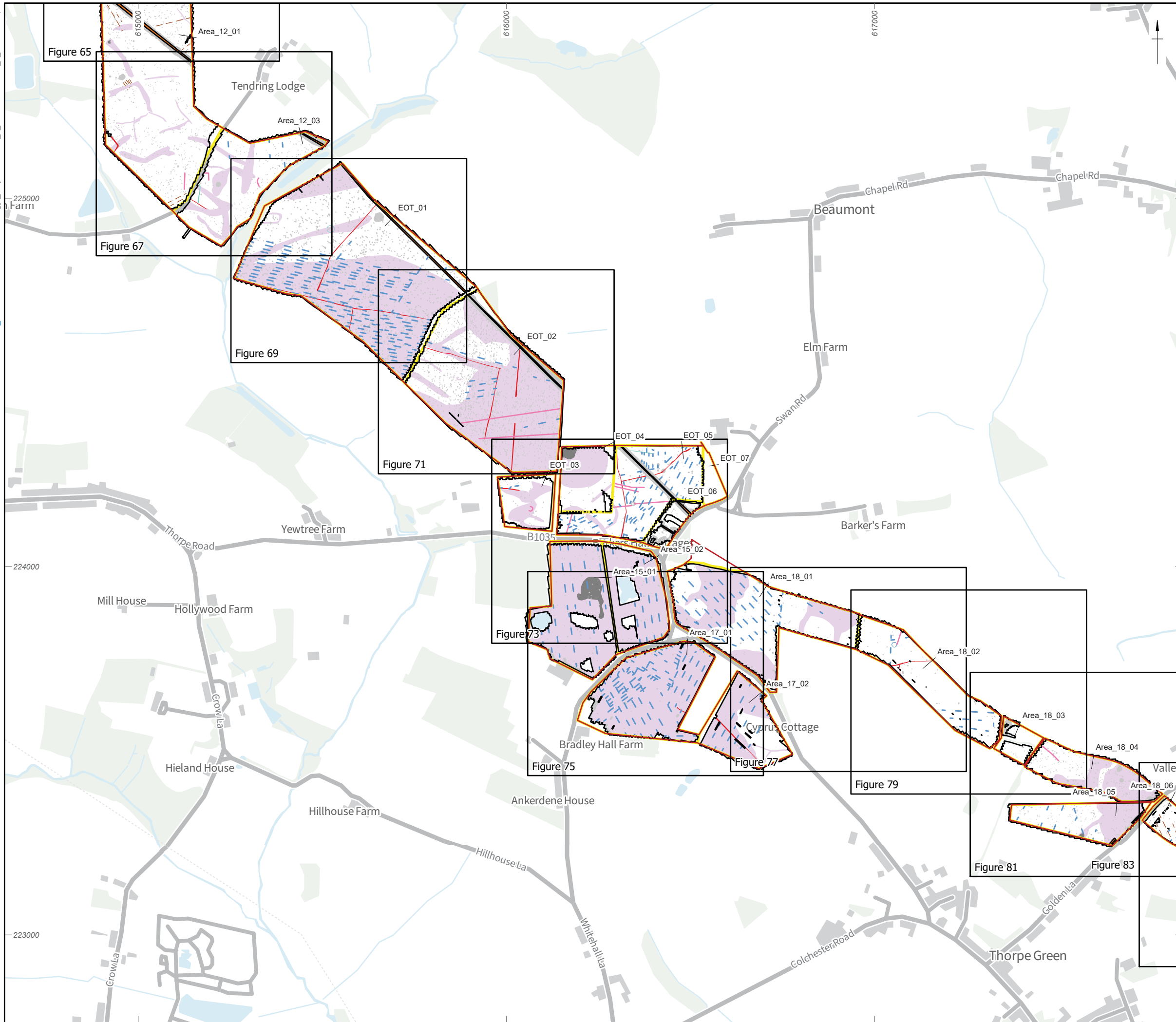
Figure 9: Gradiometer survey results: overview interpretation plot (Area 12, East of Tendring, Area 15,
