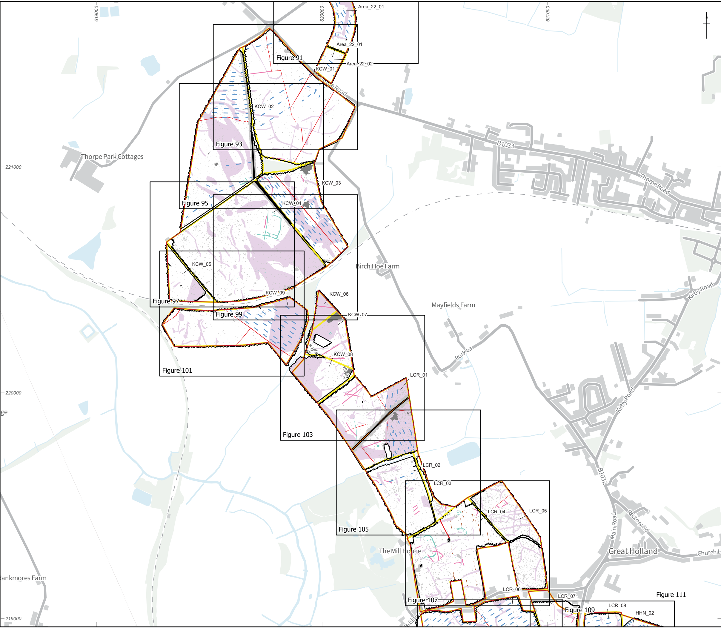
Figure 13: Gradiometer survey results: overview interpretation plot Kirby Cross West, Little Clacton Road)
