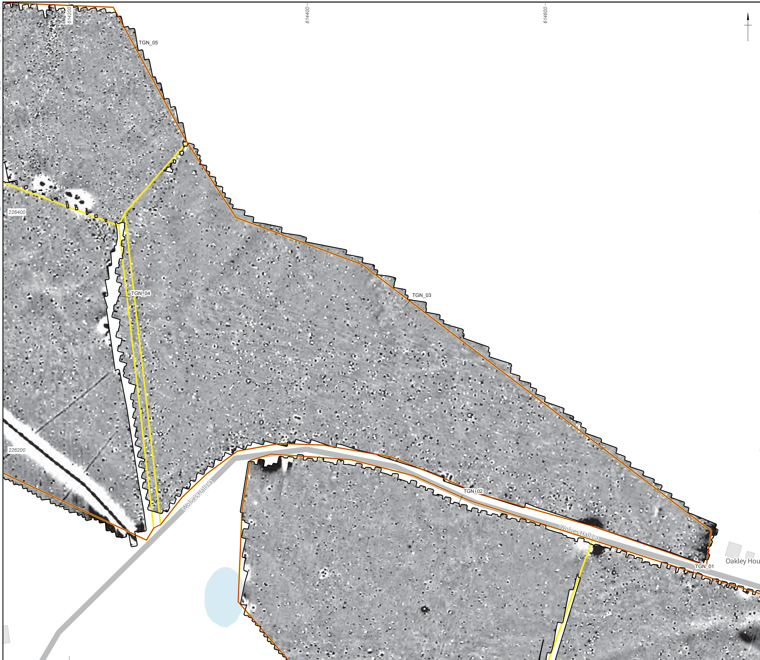
Figure 60: Gradiometer survey results: grayscale plot (TGN_02, TGN_05, TGN_01, TGN_04, TGN_03)
