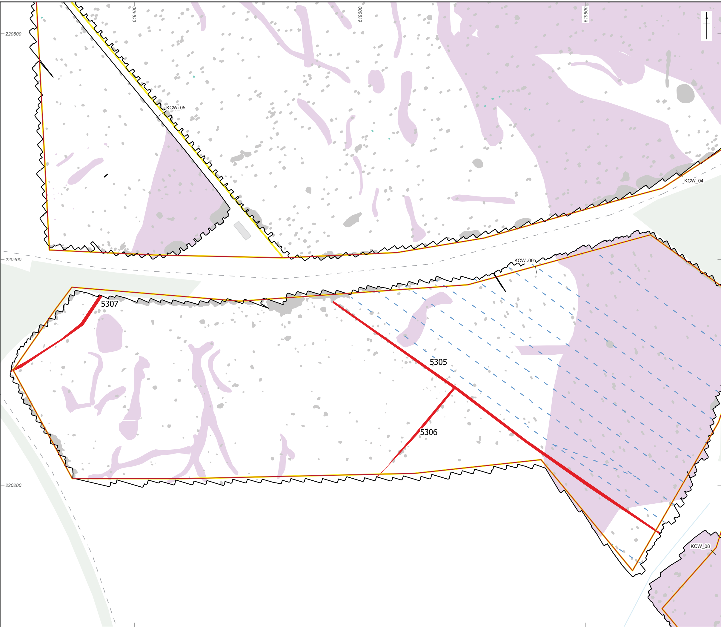
Figure 101: Gradiometer survey results: interpretation (KCW_04, KCW_09, KCW_08, KCW_05)
