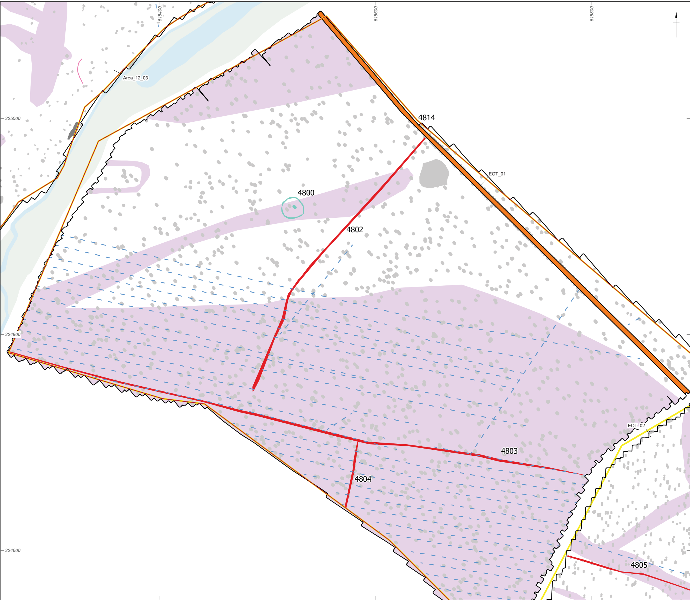
Figure 69: Gradiometer survey results: interpretation (EOT_02, EOT_01, Area_12_03)
