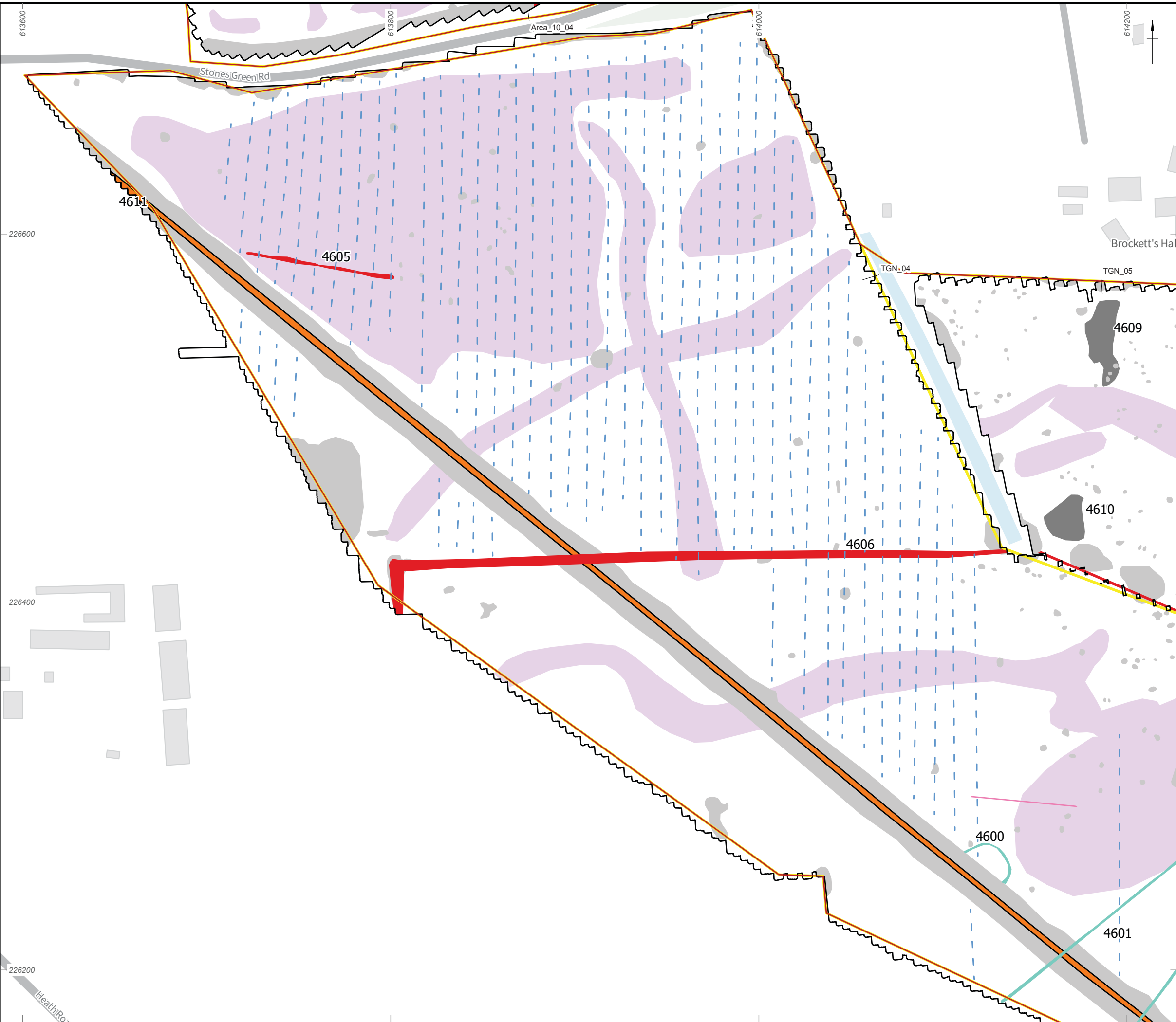
Figure 59: Gradiometer survey results: interpretation (TGN_05, TGN_04, Area_10_04)
