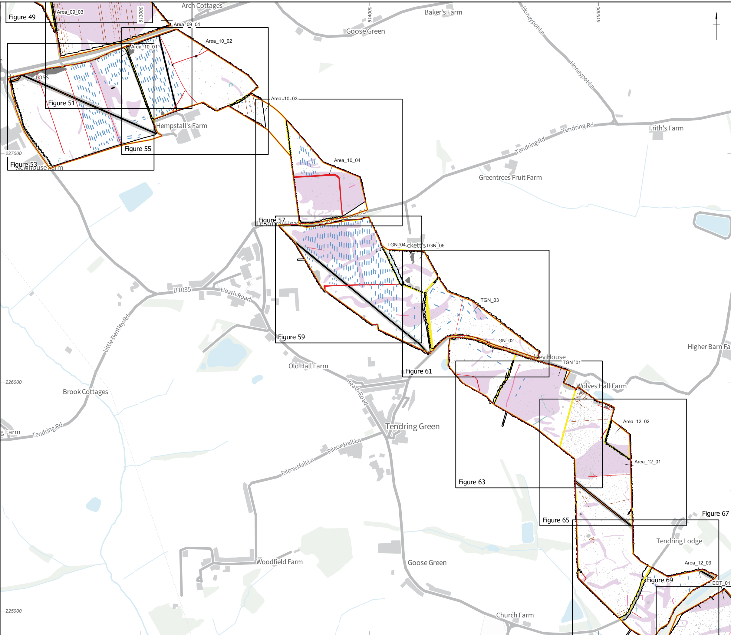
Figure 7: Gradiometer survey results: overview interpretation plot (Area 10, Tendring Green North, Area
