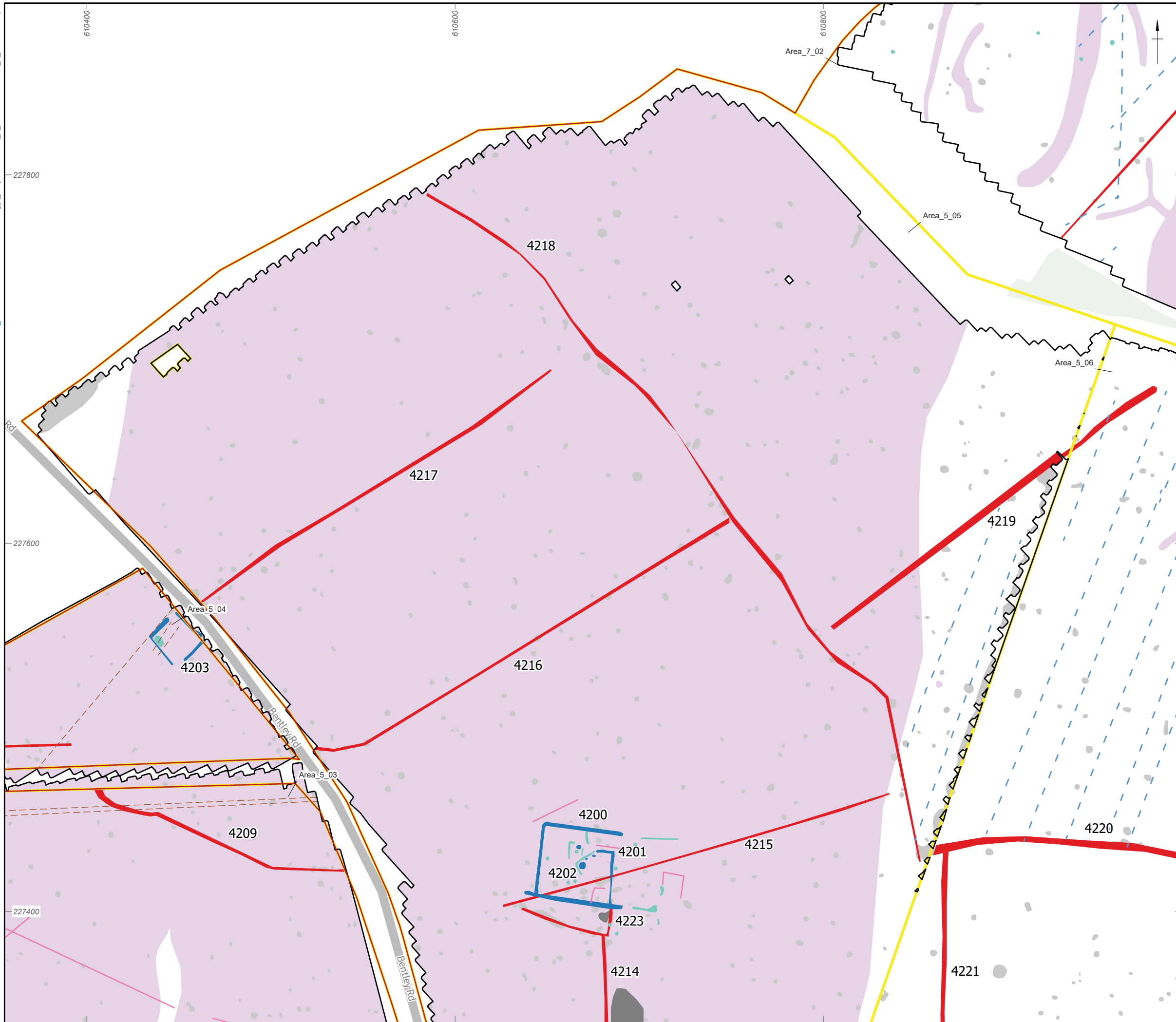
Figure 37: Gradiometer survey results: interpretation (Area_5_06, Area_5_05, Area_7_02, Area_5_03, Area_5_04)
