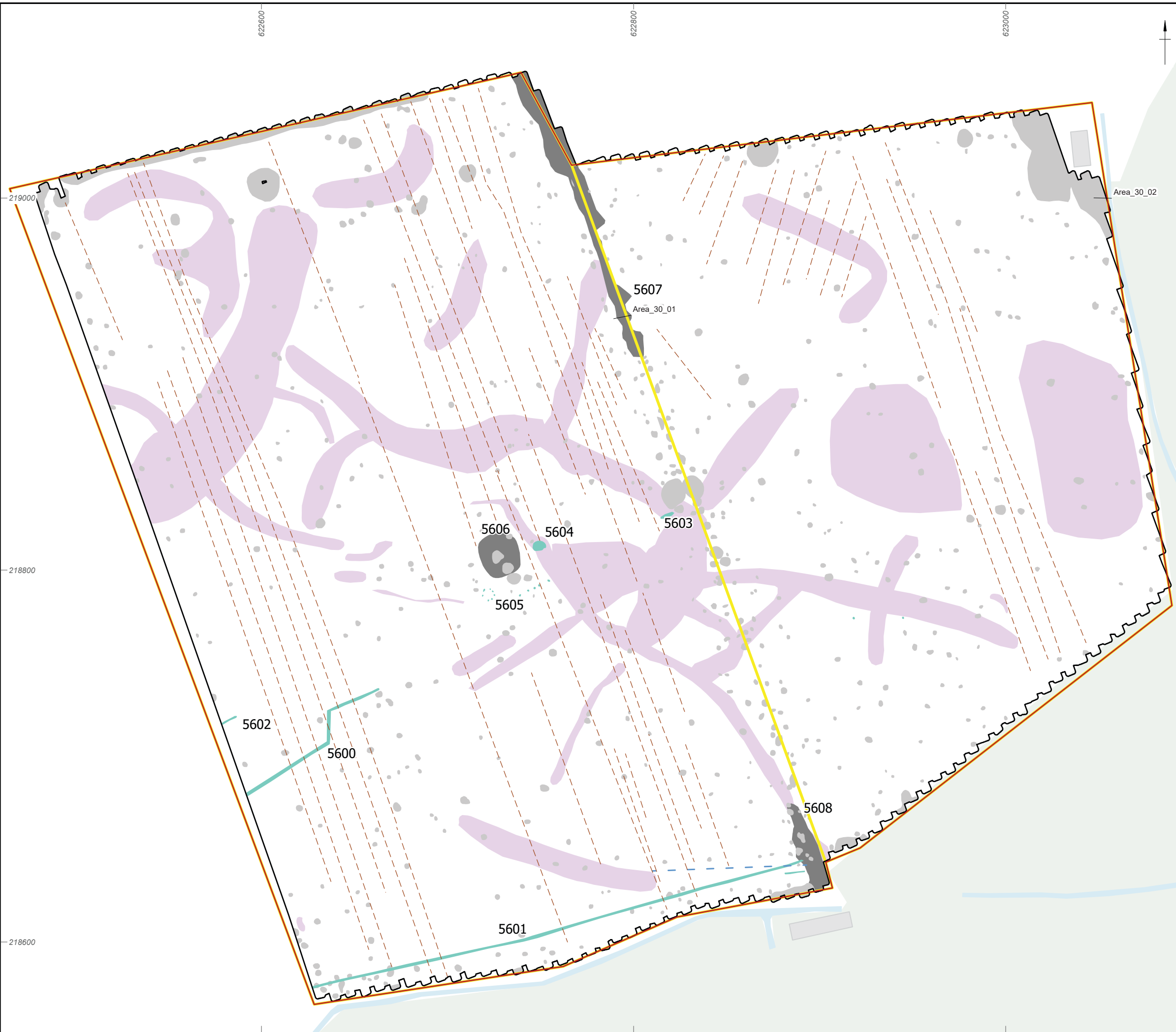
Figure 119: Gradiometer survey results: interpretation (Area_30_01, Area_30_02)
