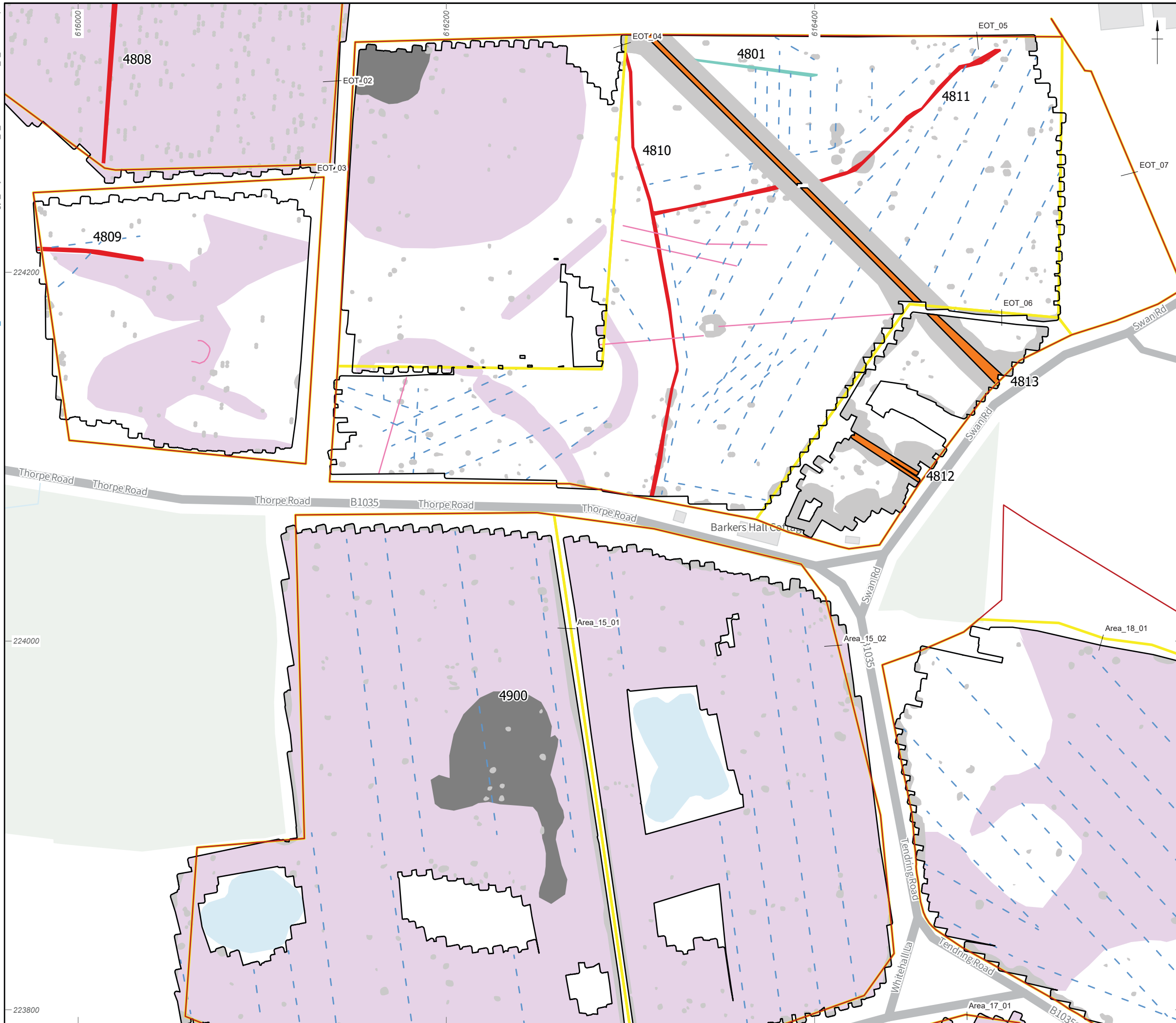
Figure 73: Gradiometer survey results: interpretation (EOT_03, EOT_02, EOT_07, EOT_06, EOT_04, EOT_05, Area_15_01, Area_15_02, Area_17_01, Area_18_01)
