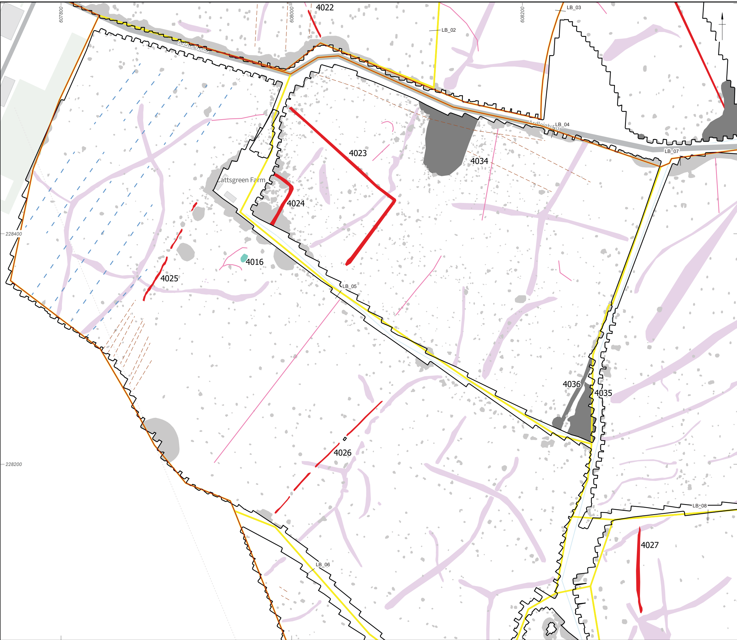
Figure 23: Gradiometer survey results: interpretation (LB_03, LB_07, LB_04, LB_05, LB_08, LB_06, LB_02)
