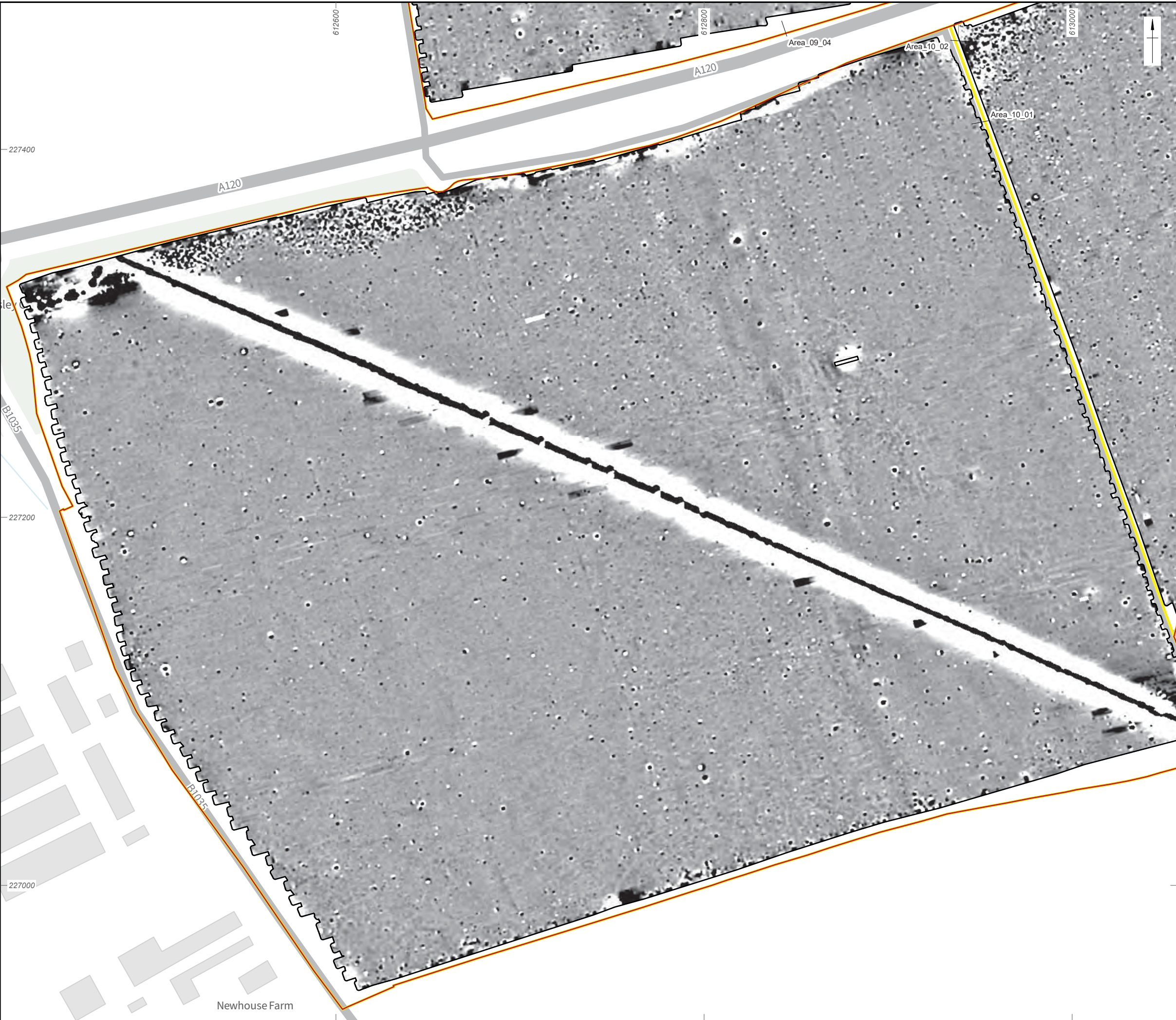
Figure 52: Gradiometer survey results: greyscale plot (Area_09_04, Area_10_02, Area_10_01)
