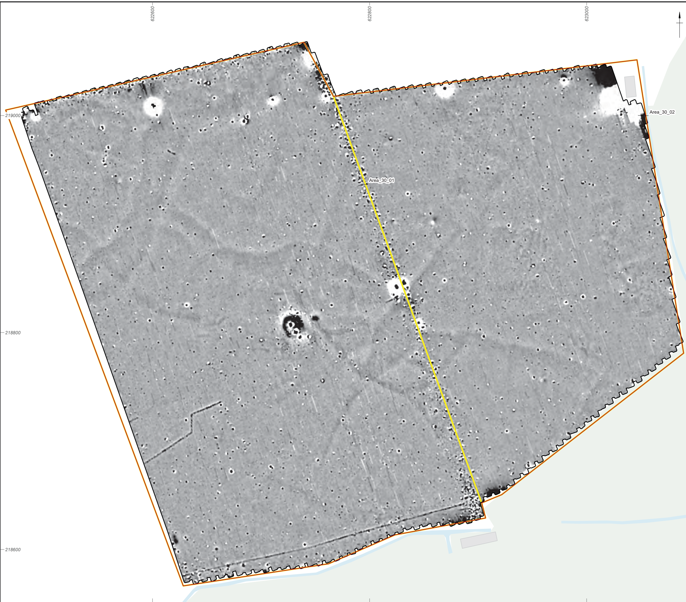
Figure 118: Gradiometer survey results: greyscale plot (Area_30_01, Area_30_02)
