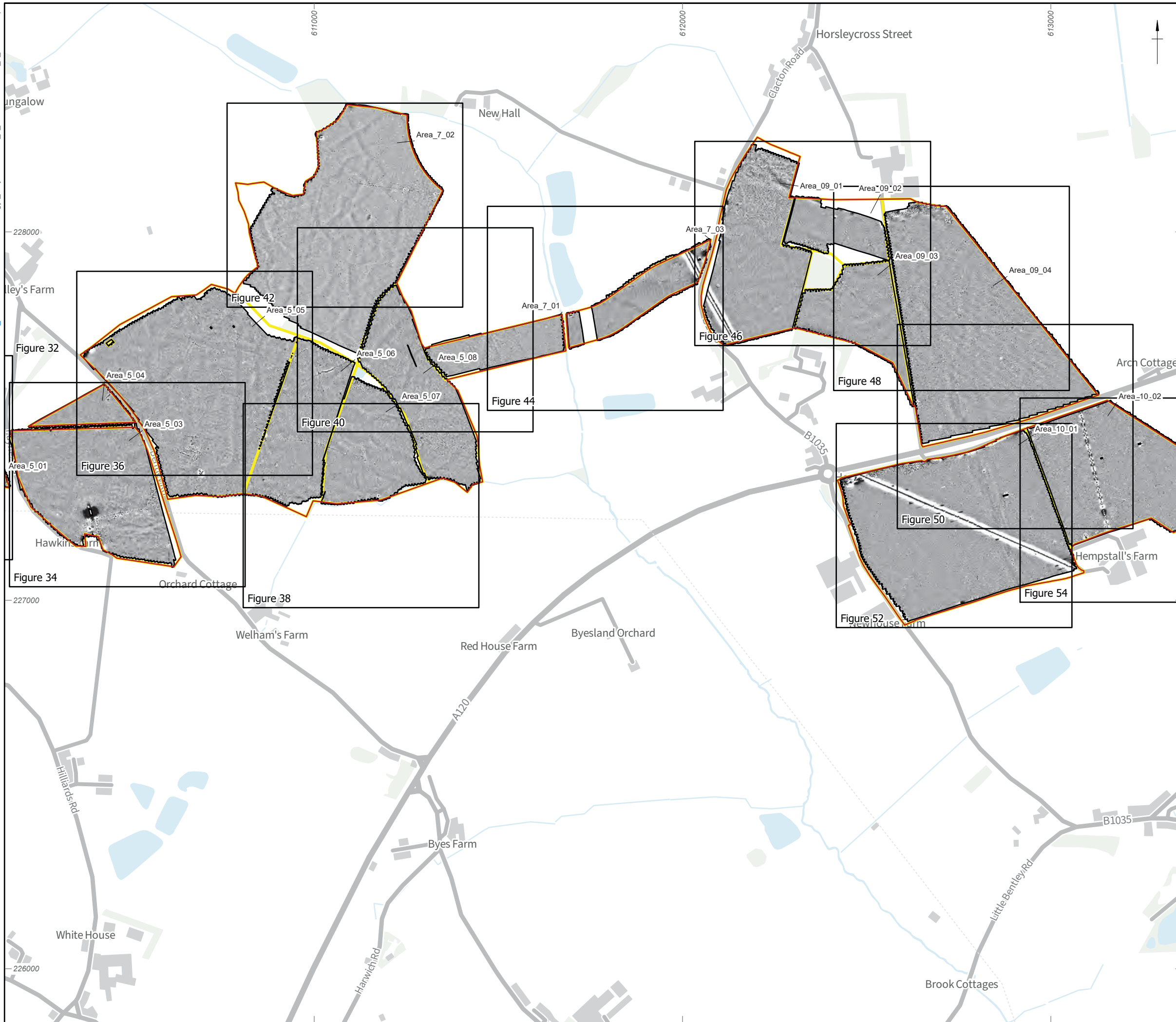
Figure 4: Gradiometer survey results: overview greyscale plot (Area 5, Area 7, Area 9, Area 10)
