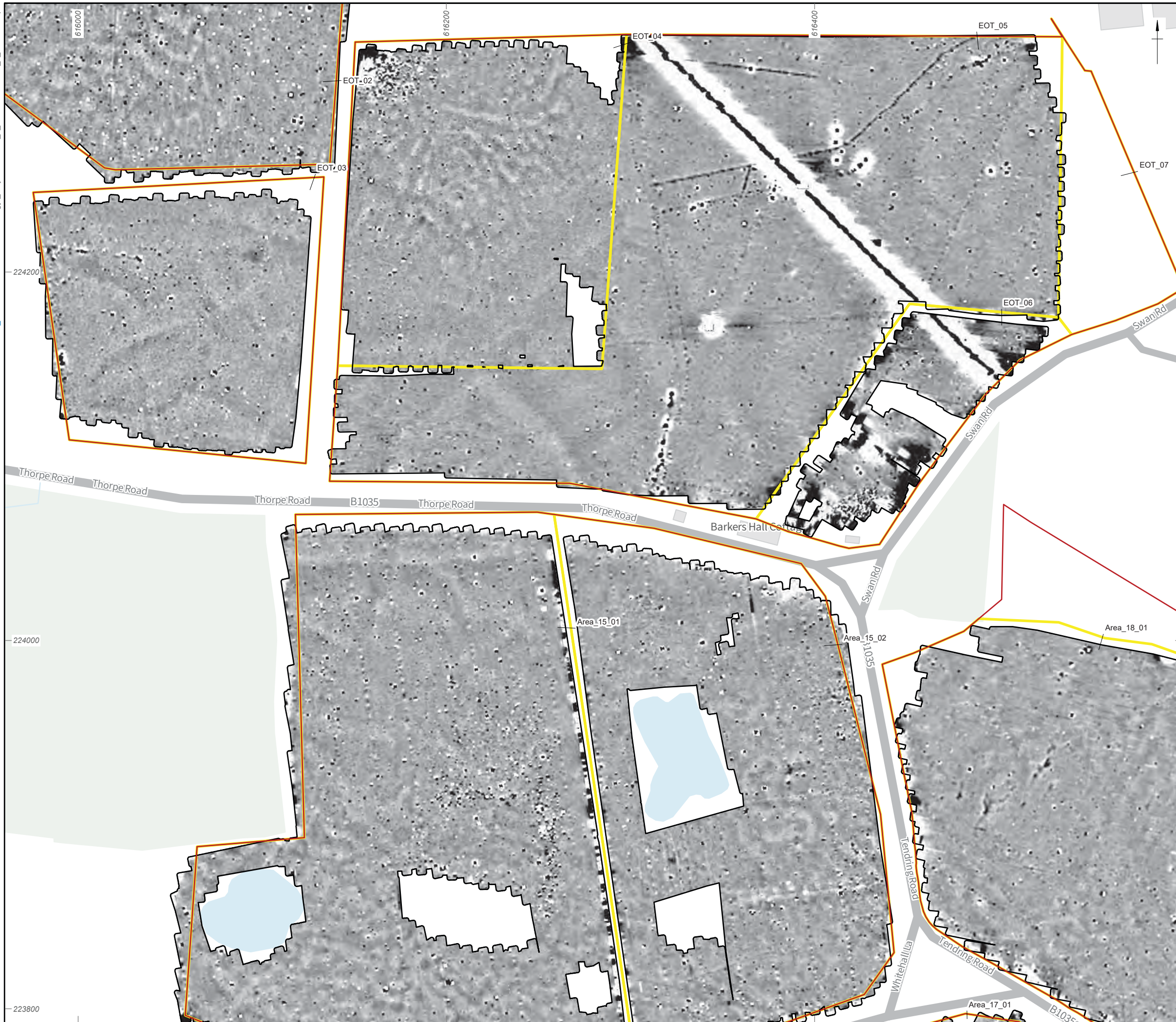
Figure 72: Gradiometer survey results: grayscale plot (EOT_03, EOT_02, EOT_07, EOT_06, EOT_04, EOT_05, Area_15_01, Area_15_02, Area_17_01, Area_18_01)
