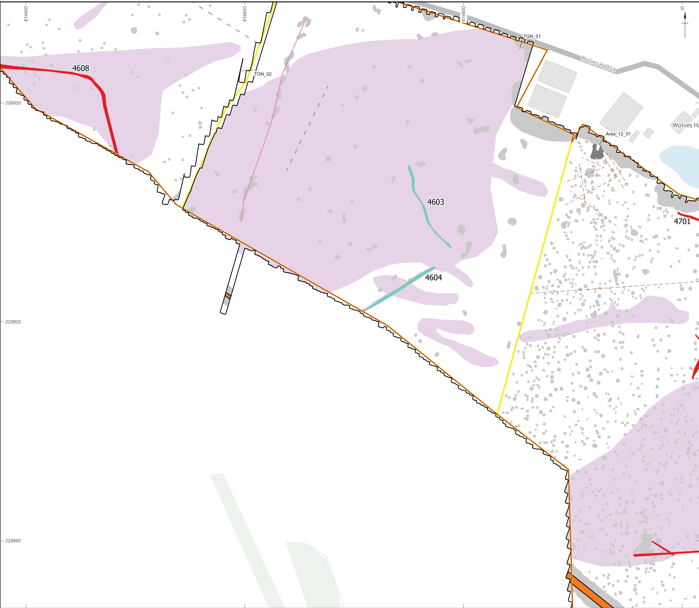
Figure 63: Gradiometer survey results: interpretation (TGN_02, TGN_01, Area_12_01)
