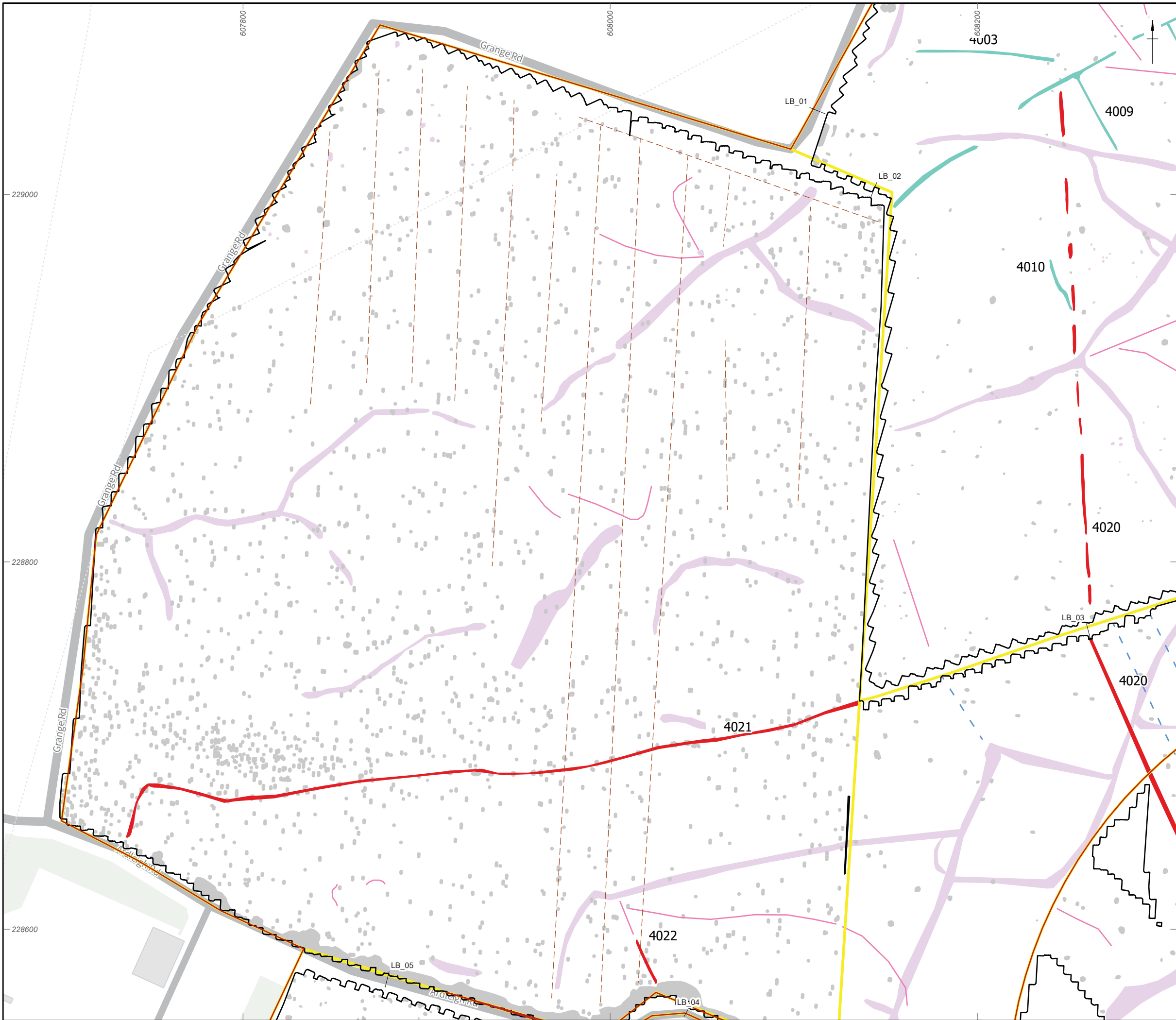
Figure 19: Gradiometer survey results: interpretation (LB_03, LB_04, LB_01, LB_05, LB_02)
