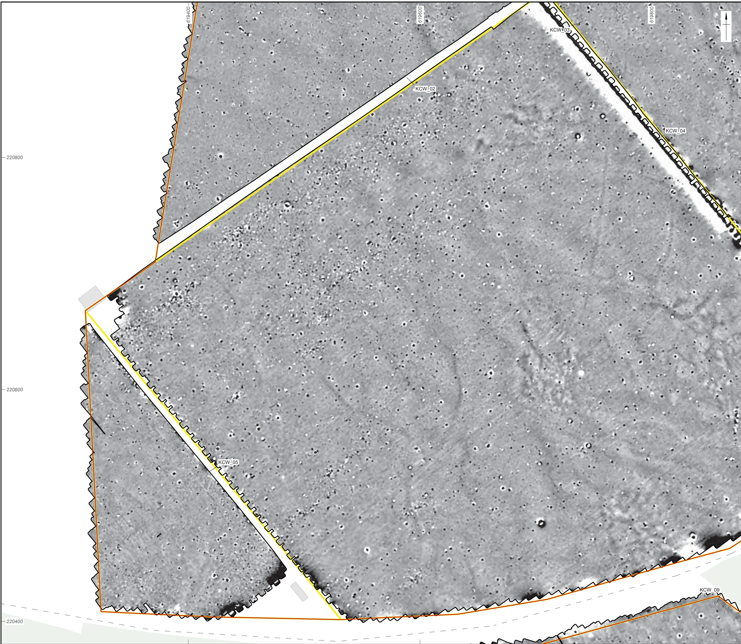
Figure 96: Gradiometer survey results: grayscale plot (KCW_04, KCW_09, KCW_03, KCW_02, KCW_05)
