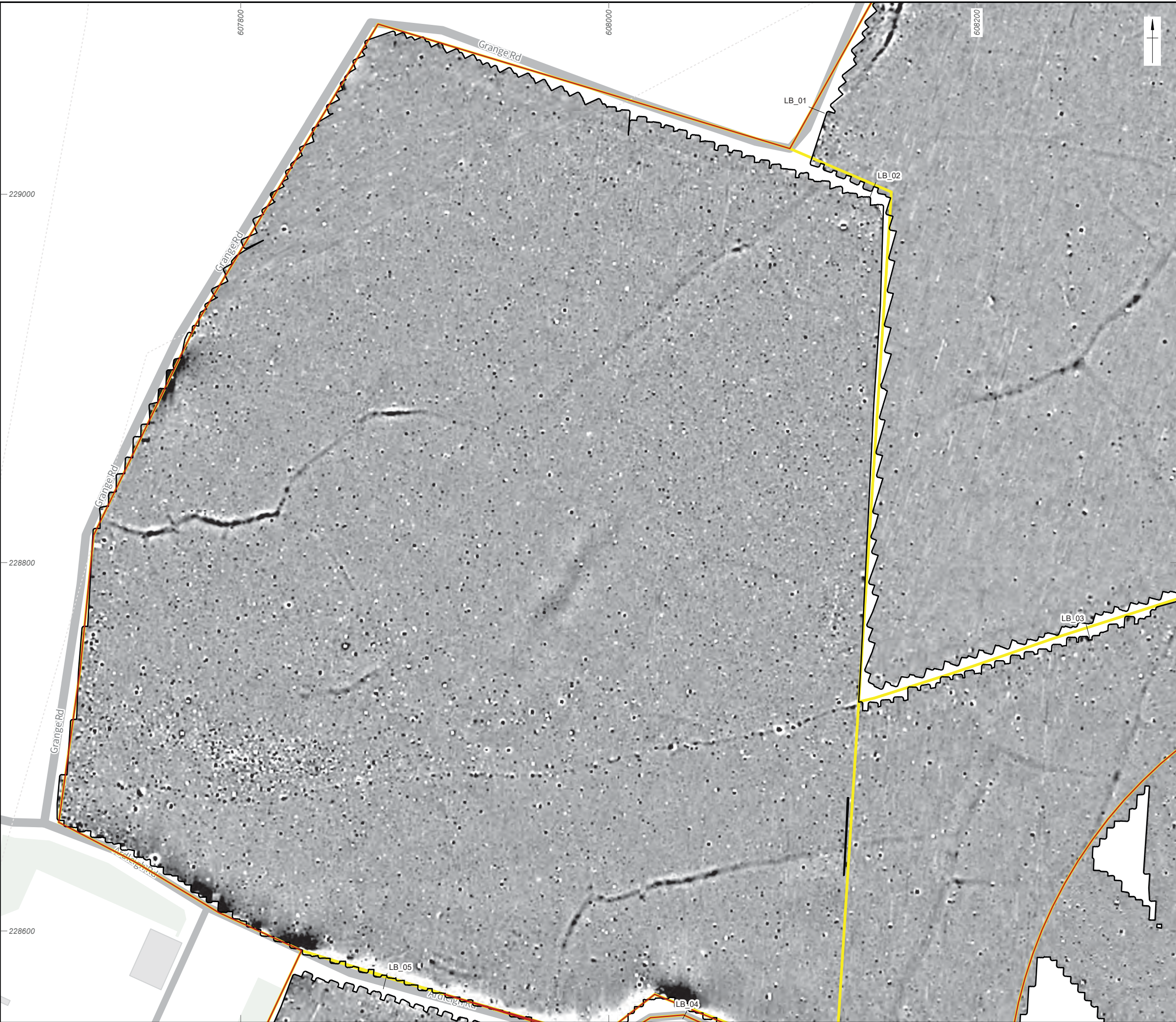
Figure 18: Gradiometer survey results: greyscale plot (LB_03, LB_04, LB_01, LB_05, LB_02)
