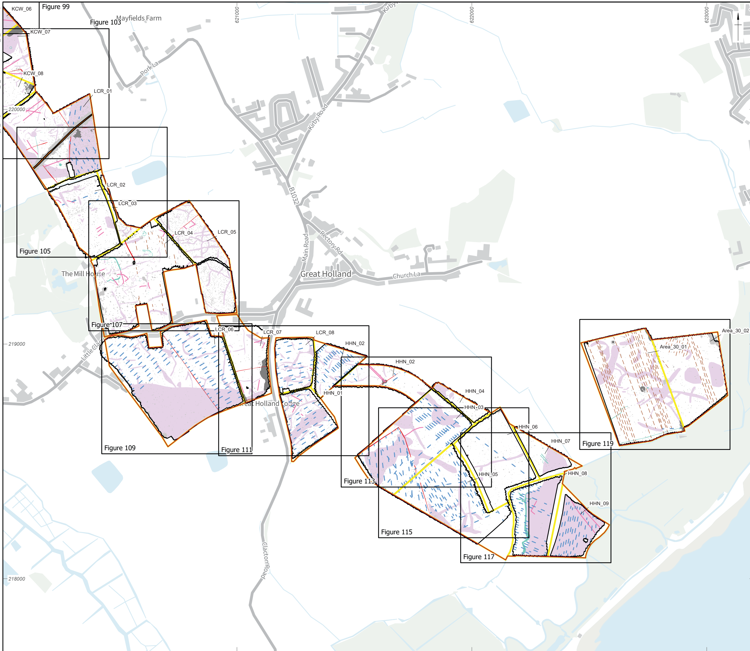
Figure 15: Gradiometer survey results: overview interpretation plot Little Clacton Road, Holadn Haven
