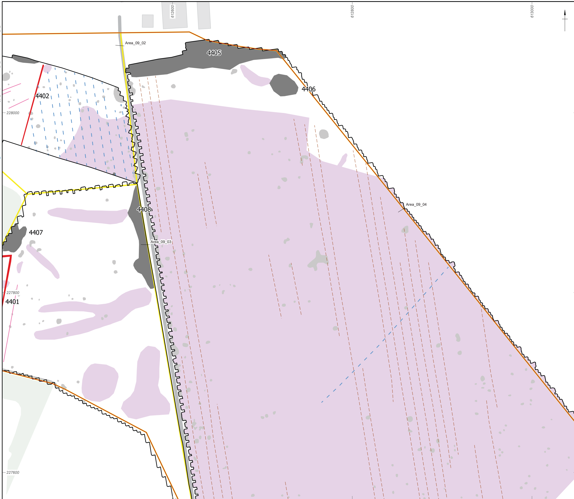
Figure 49: Gradiometer survey results: interpretation (Area_09_04, Area_09_03, Area_09_02)
