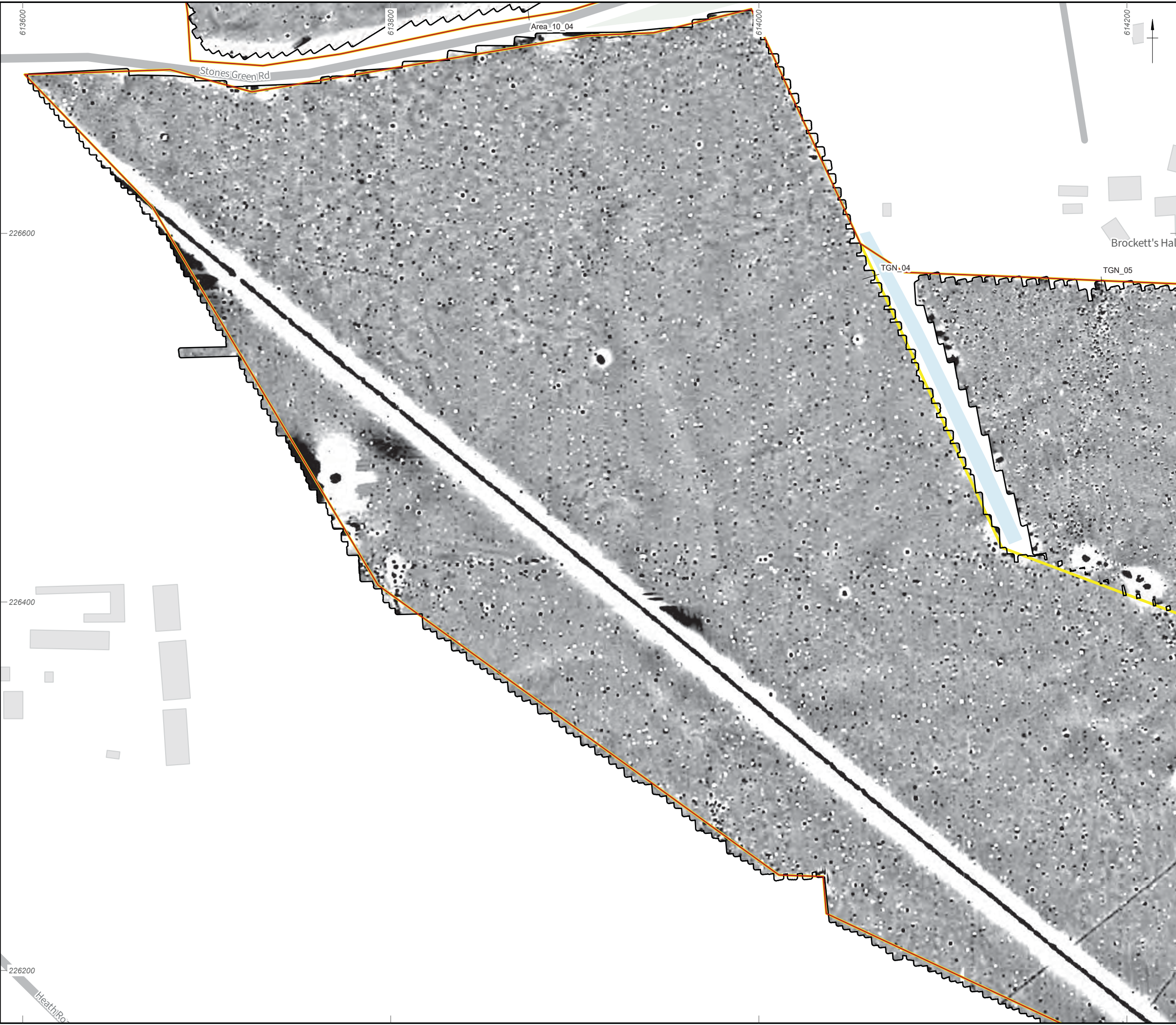
Figure 58: Gradiometer survey results: greyscale plot (TGN_05, TGN_04, Area_10_04)
