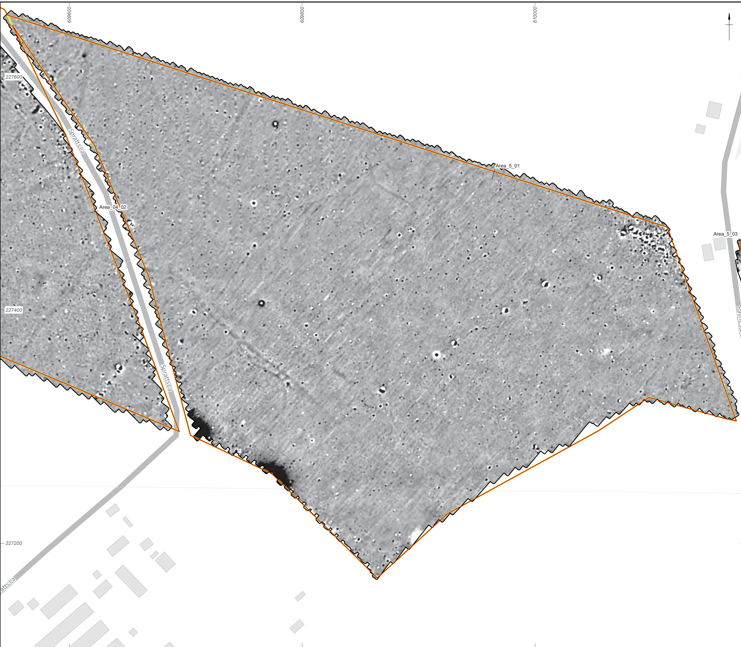
Figure 32: Gradiometer survey results: grayscale plot (Area_04_02, Area_5_01, Area_5_03)
