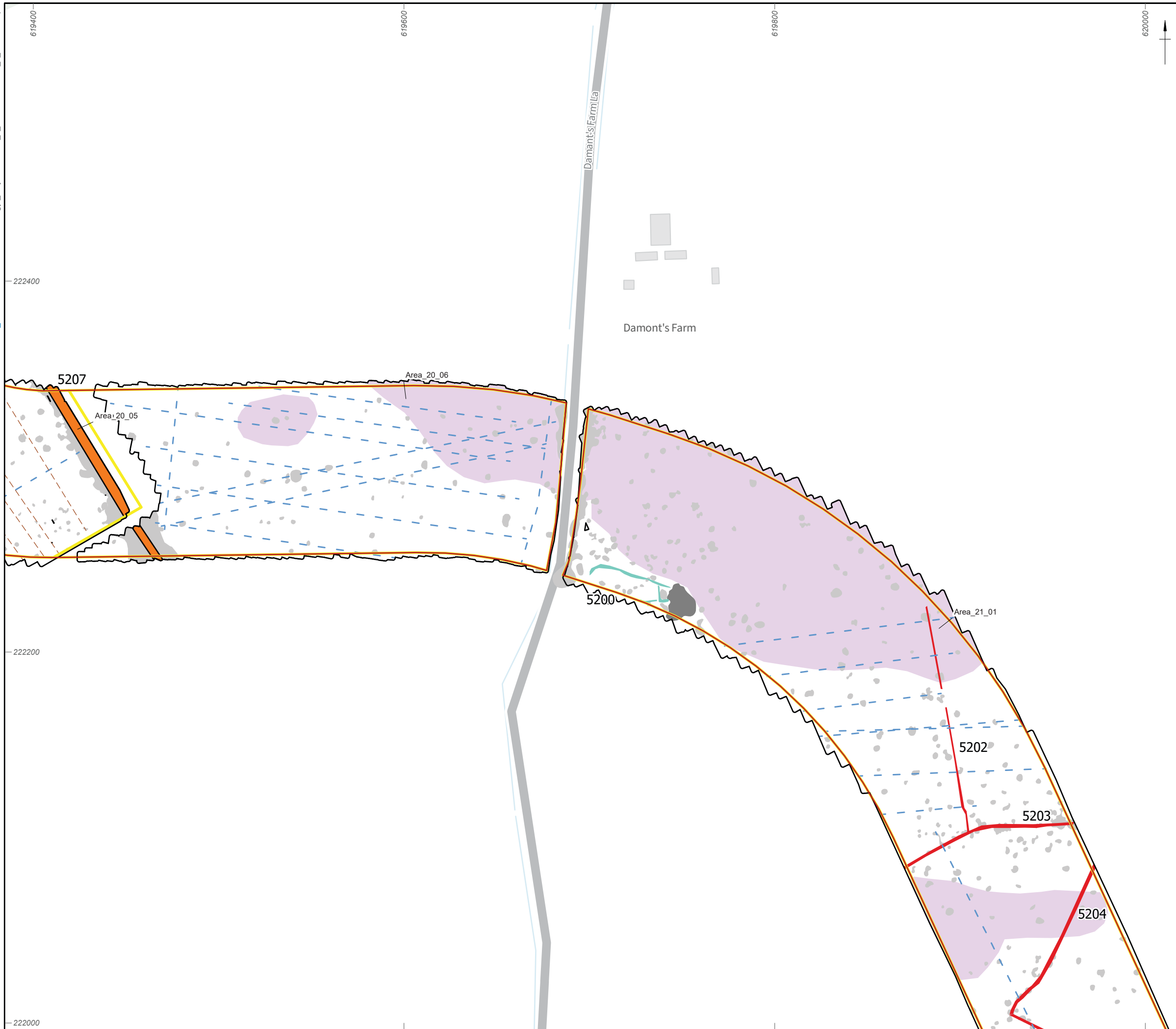
Figure 89: Gradiometer survey results: interpretation (Area_20_05, Area_20_06, Area_21_01)
