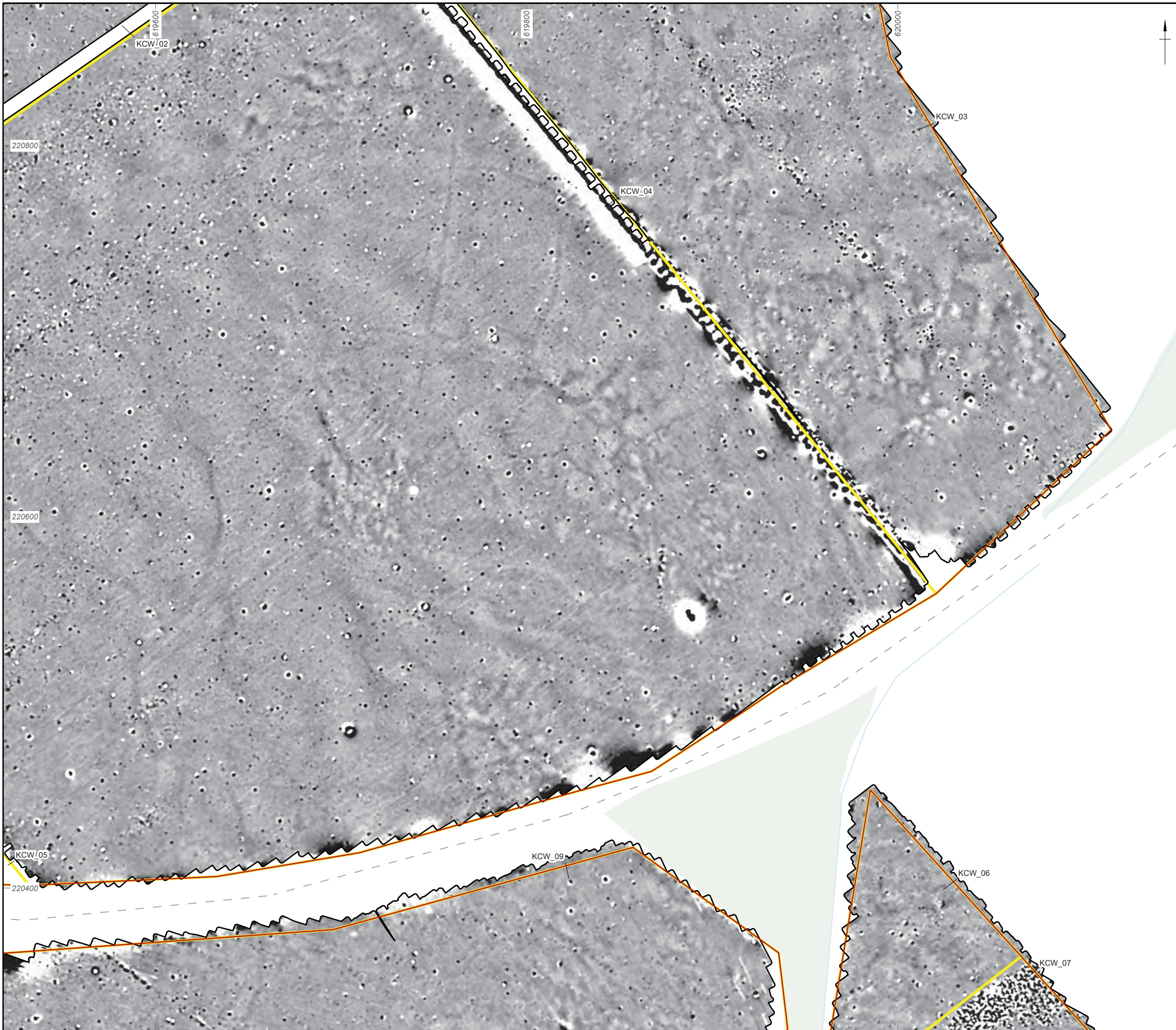
Figure 98: Gradiometer survey results: greyscale plot (KCW_04, KCW_09, KCW_03, KCW_02, KCW_06, KCW_07, KCW_05)
