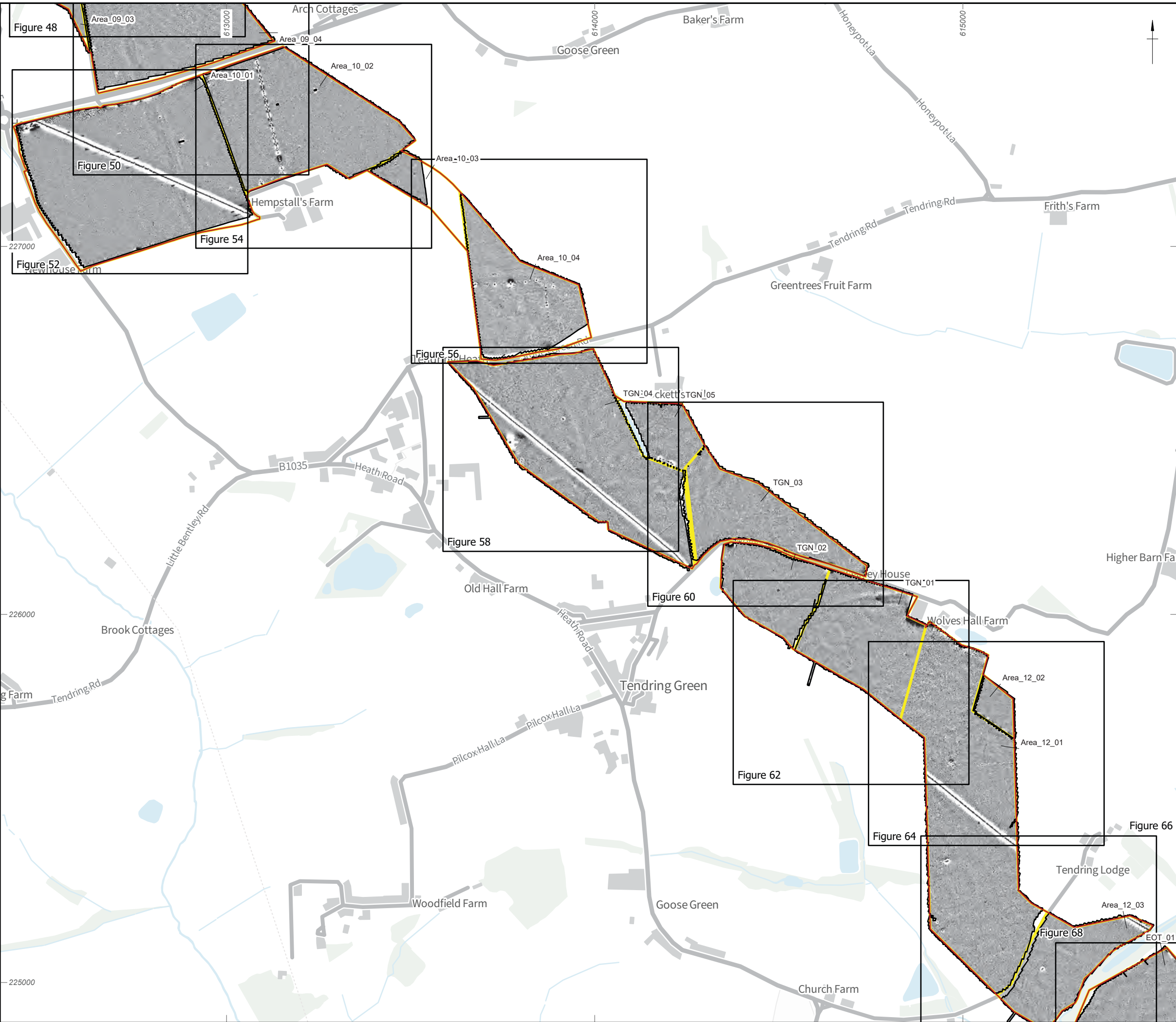
Figure 6: Gradiometer survey results: overview greyscale plot (Area 10, Tendring Green North, Area 12)
