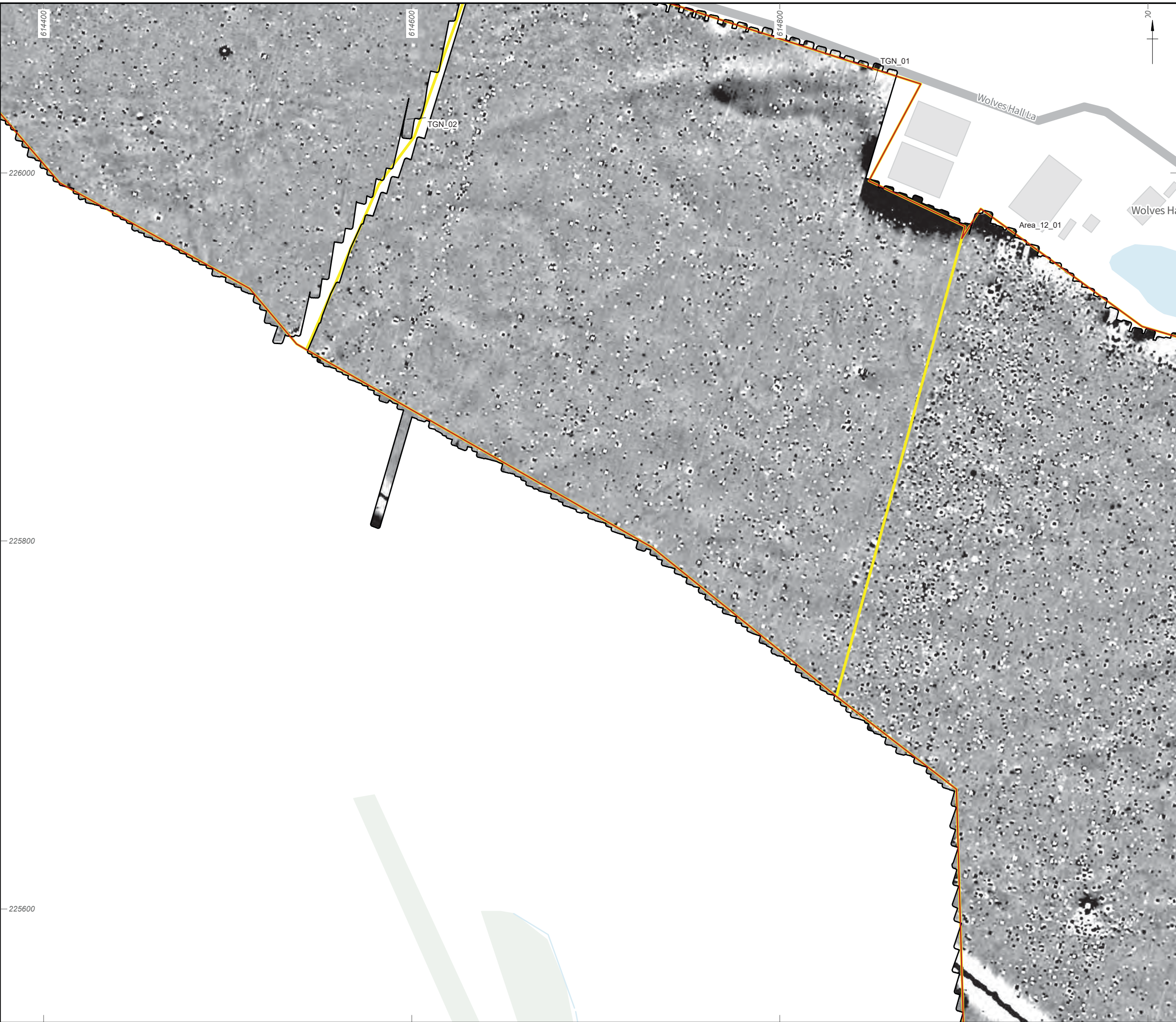
Figure 62: Gradiometer survey results: grayscale plot (TGN_02, TGN_01, Area_12_01)
