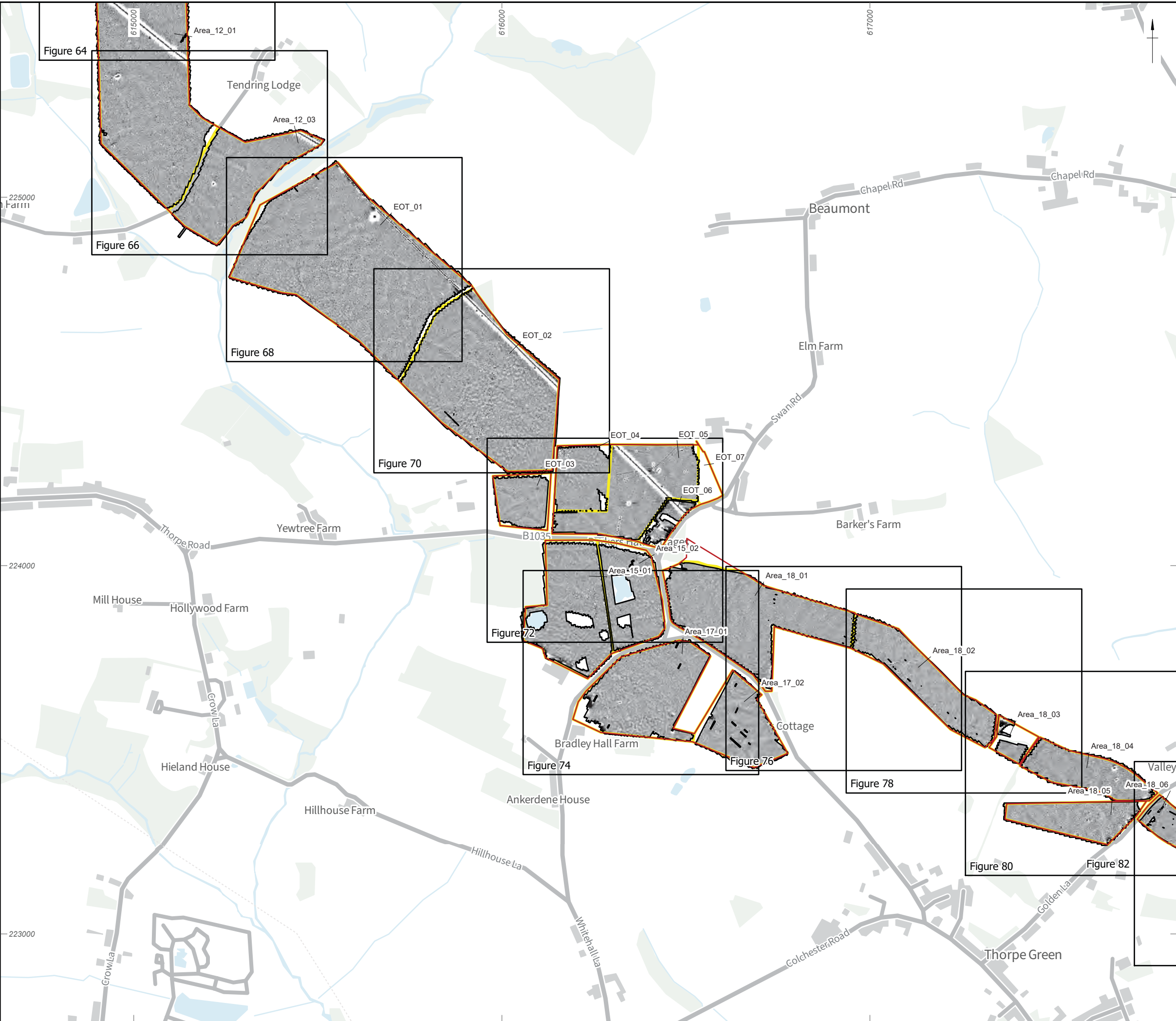
Figure 8: Gradiometer survey results: overview greyscale plot (Area 12, East of Tendring, Area 15, Area 17, Area 18)
