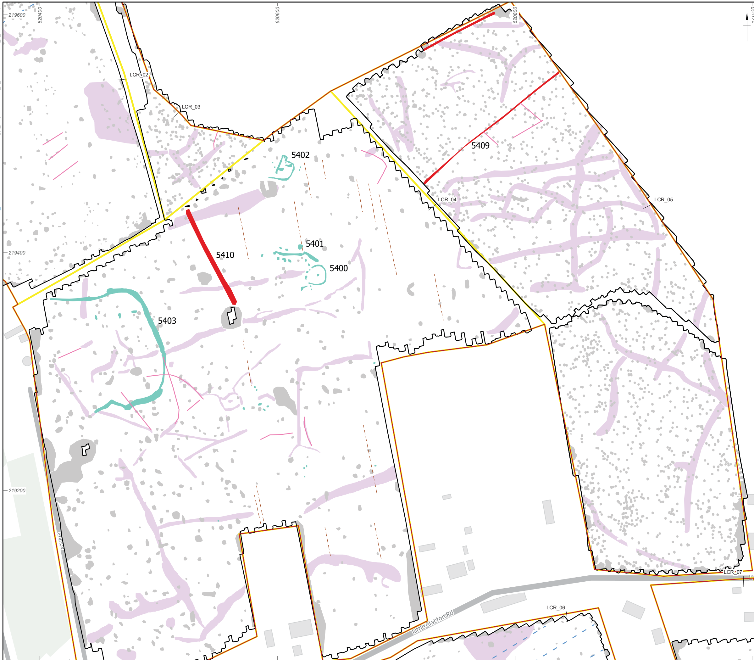
Figure 107: Gradiometer survey results: interpretation (LCR_07, LCR_06, LCR_05, LCR_04, LCR_02, LCR_03)
