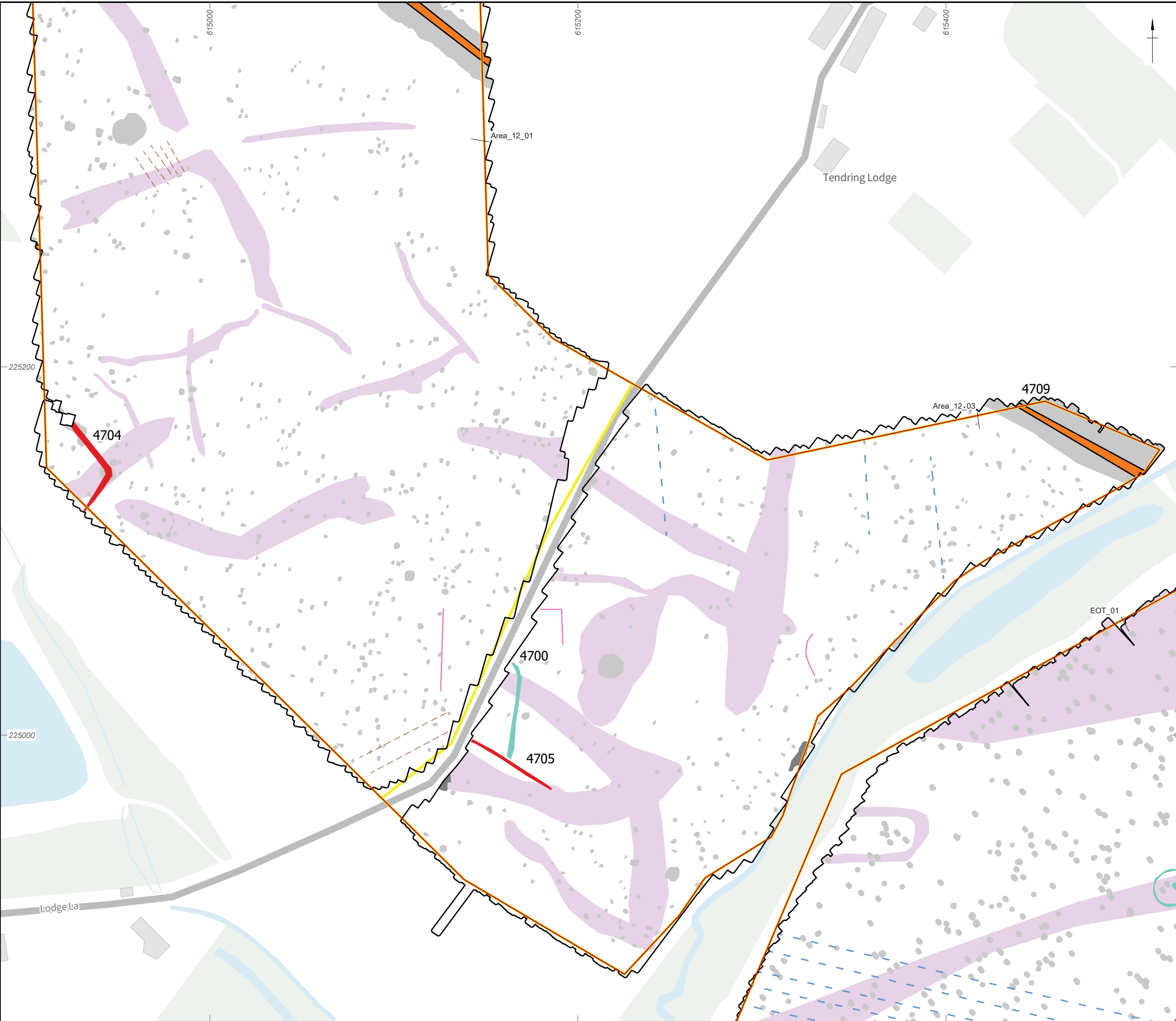
Figure 67: Gradiometer survey results: interpretation (EOT_01, Area_12_01, Area_12_03)
