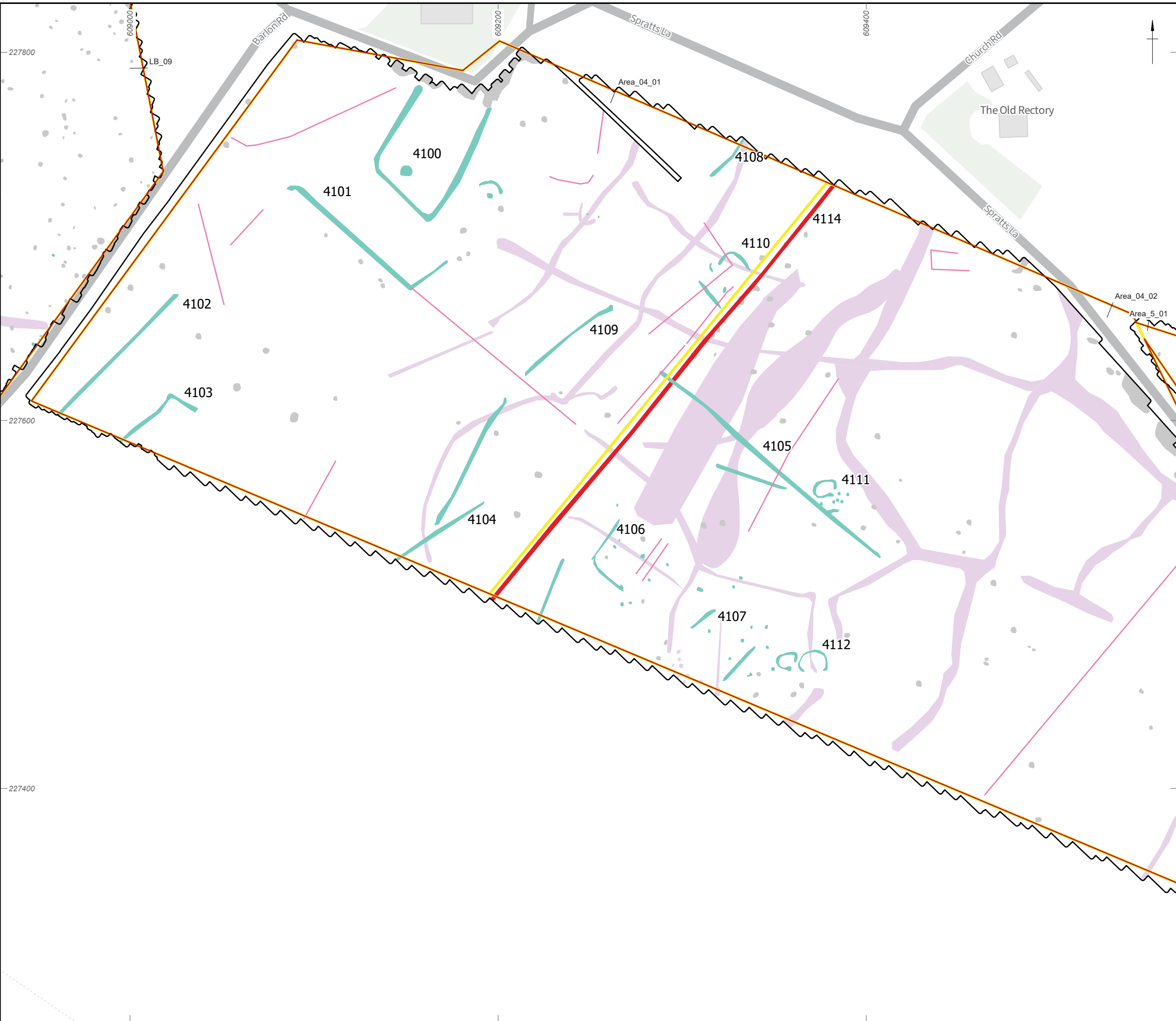
Figure 31: Gradiometer survey results: interpretation (LB_09, Area_04_01, Area_04_02, Area_5_01)
