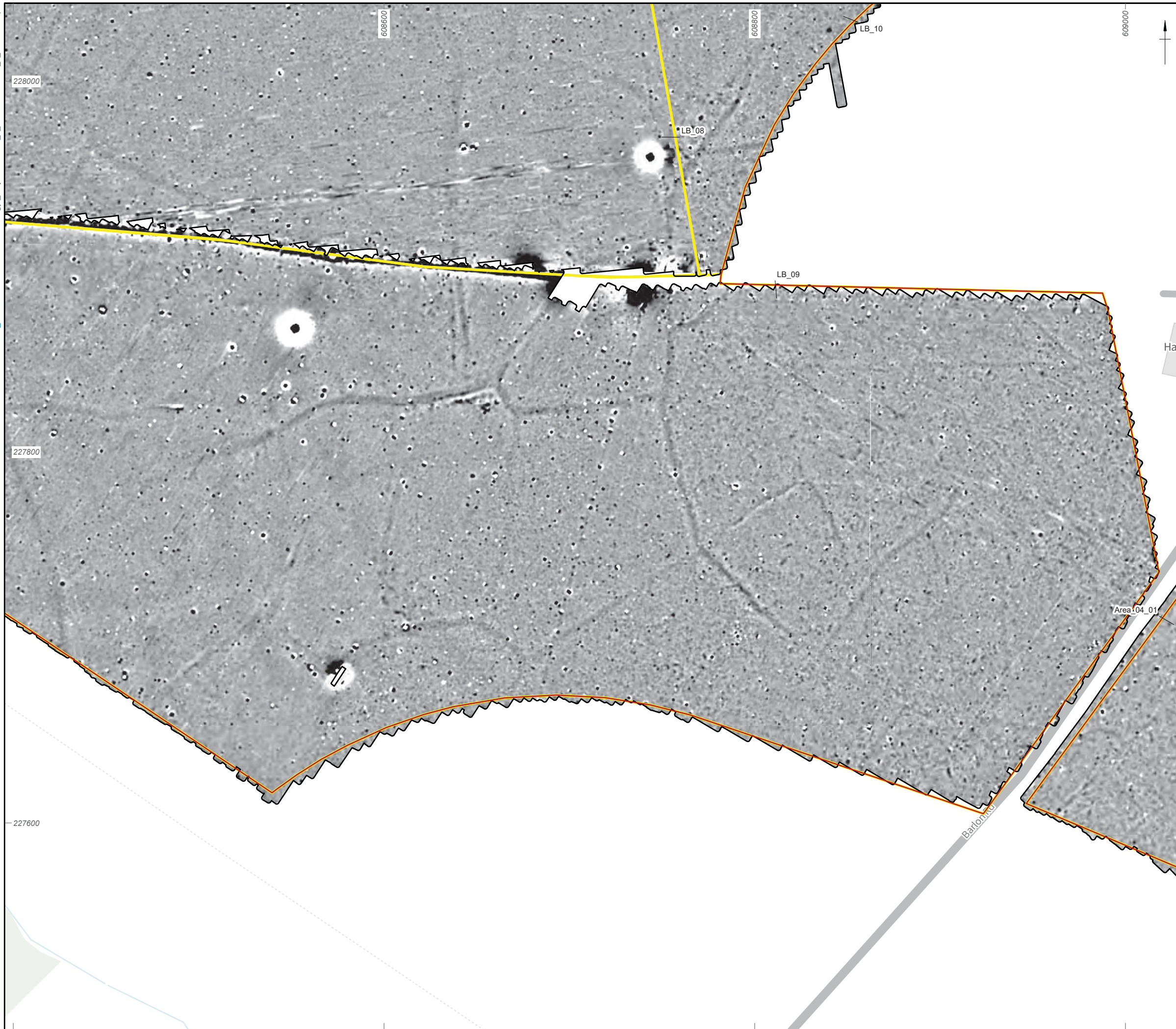
Figure 28: Gradiometer survey results: greyscale plot (LB_08, LB_10, LB_09, Area_04_01)
