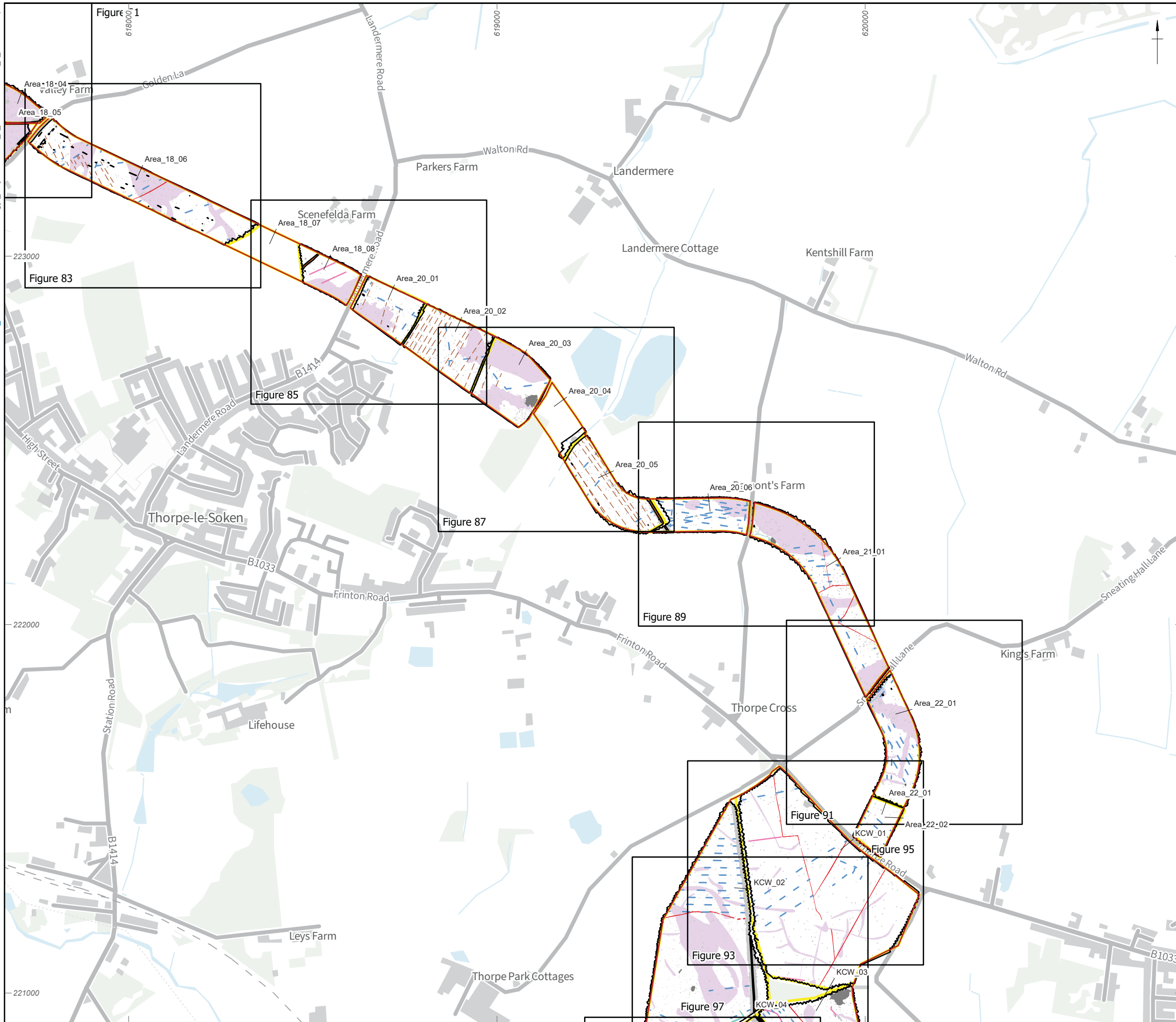
Figure 11: Gradiometer survey results: overview interpretation plot (Area 18, Area 20)
