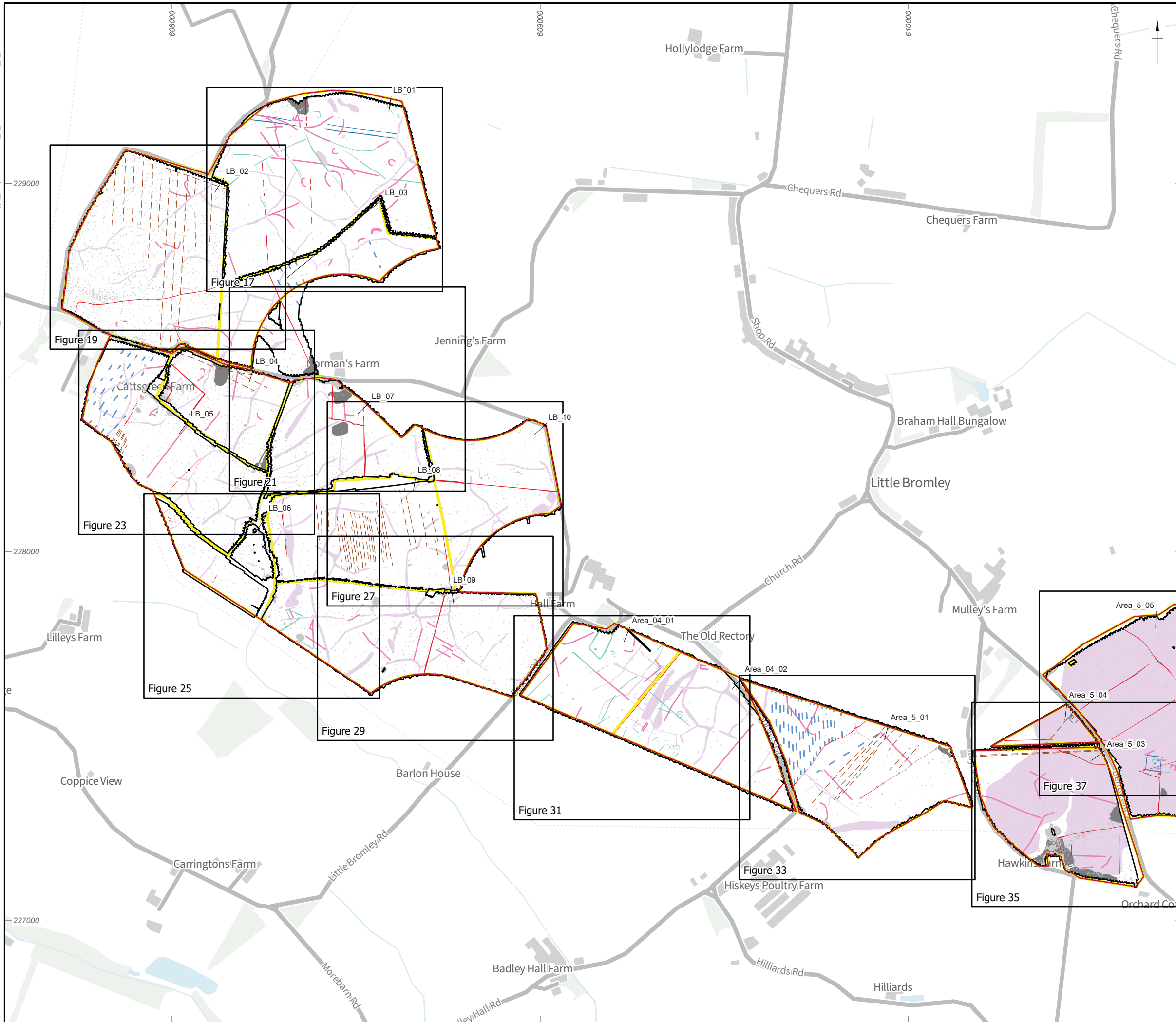
Figure 3: Gradiometer survey results: overview interpretation plot (Little Bromley, Area 4, Area 5)
