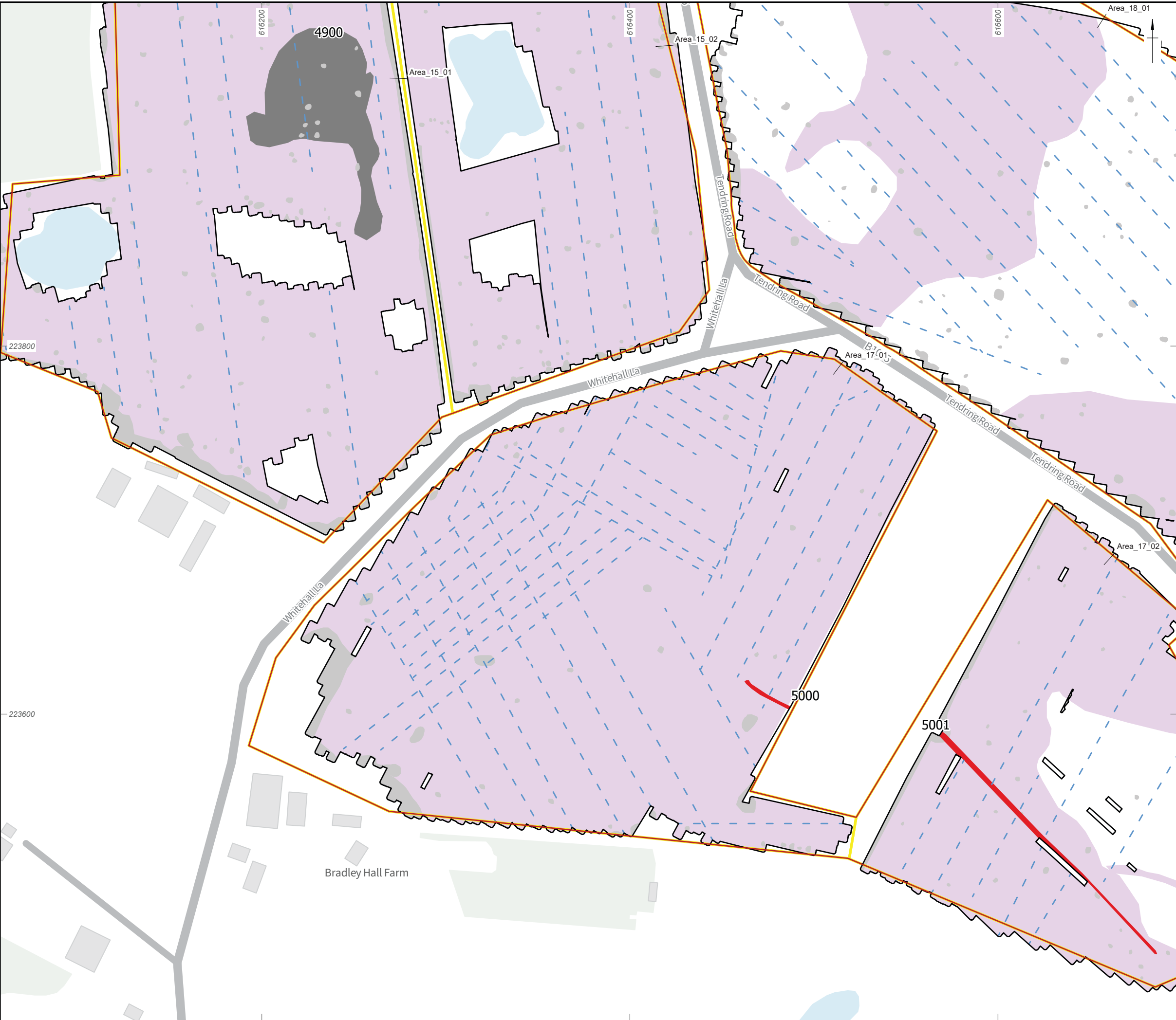
Figure 75: Gradiometer survey results: interpretation (Area_15_01, Area_15_02, Area_17_02, Area_17_01, Area_18_01)
