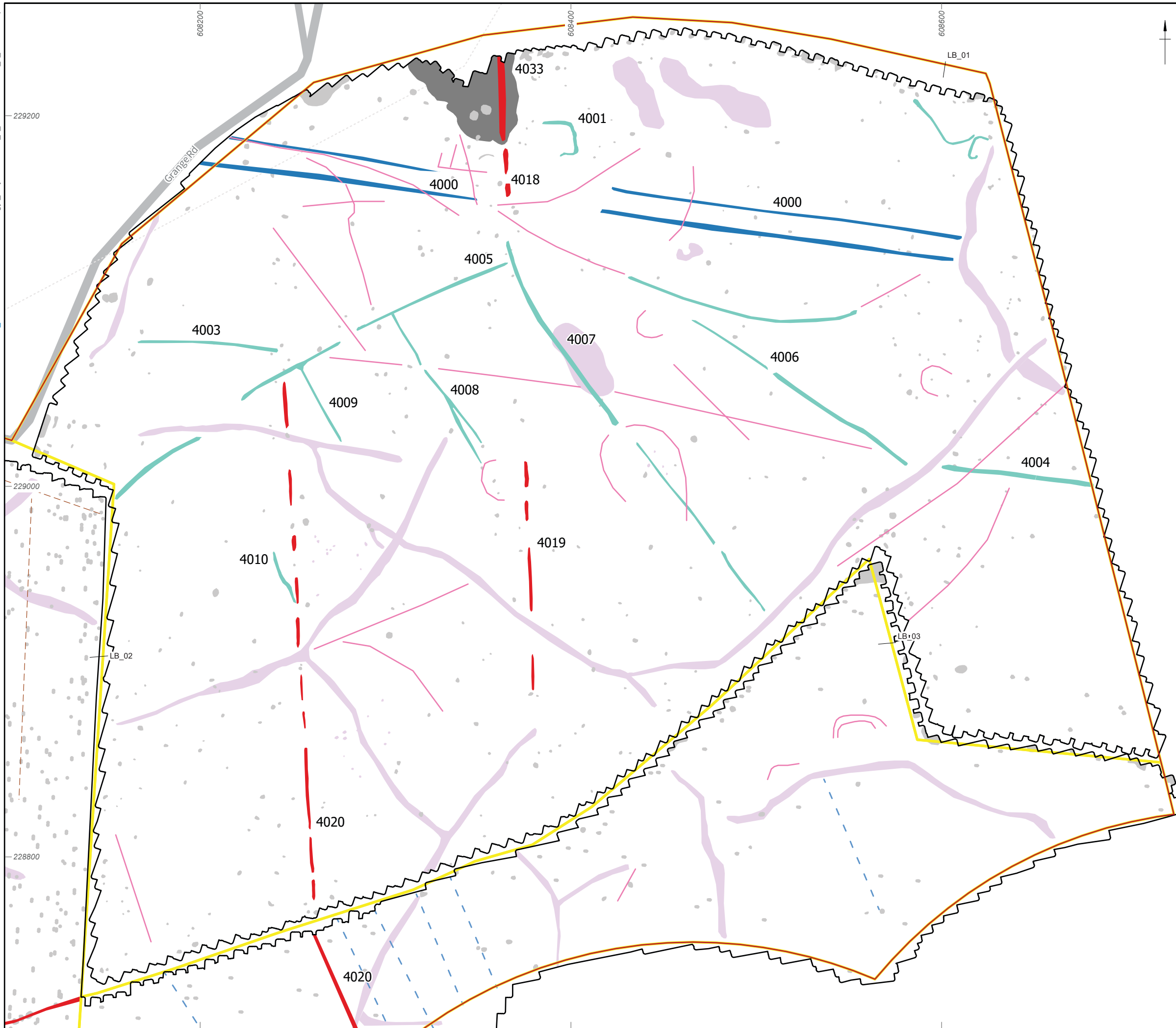
Figure 17: Gradiometer survey results: interpretation (LB_03, LB_01, LB_02)
