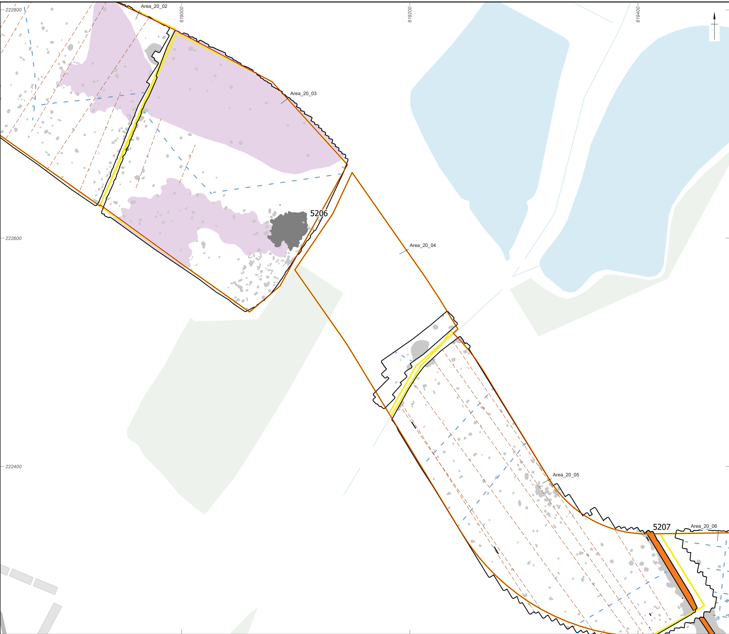
Figure 87: Gradiometer survey results: interpretation (Area_20_05, Area_20_02, Area_20_03, Area_20_06, Area_20_04)
